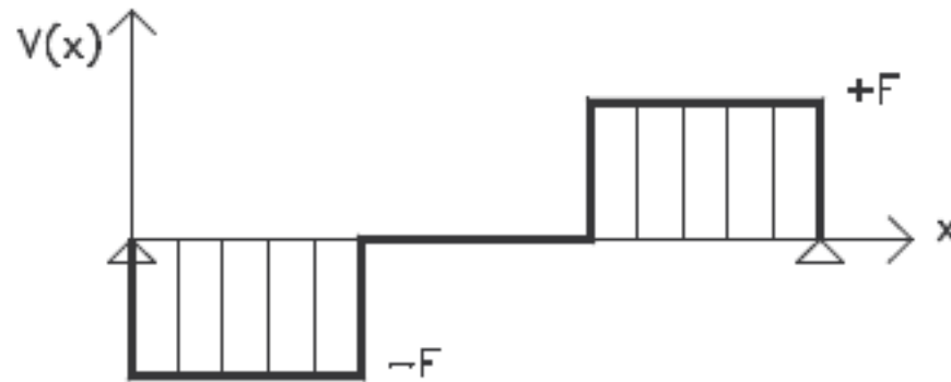
Efforts tranchants
