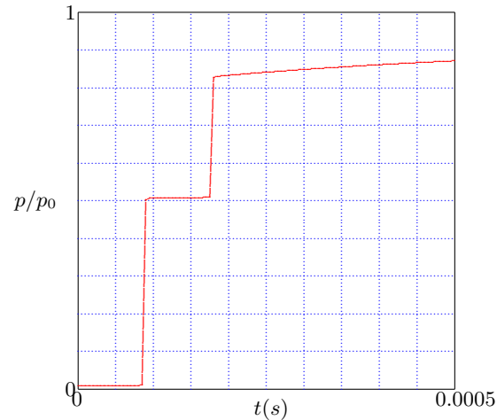
Figure 5.3: Shock wave in porous medium - Analytical solution.
