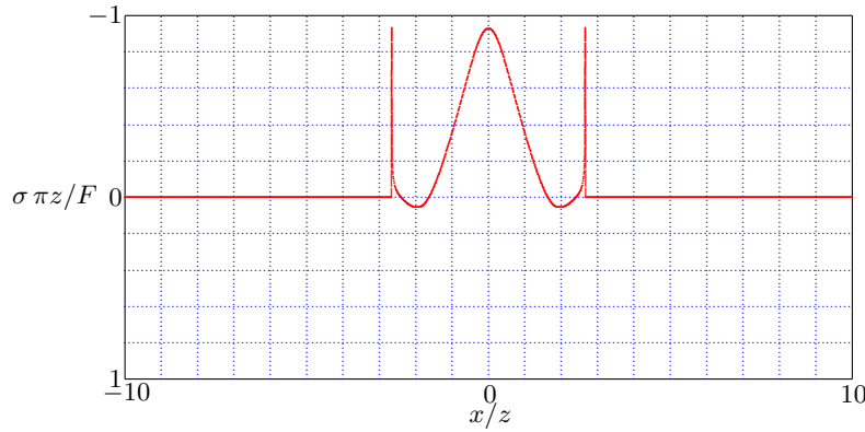
Figure 11.18: Line Load - Isotropic Stress, \nu = 0 , c_s t/z = 2 and \nu = 0 , c_s t/z = 10 .
