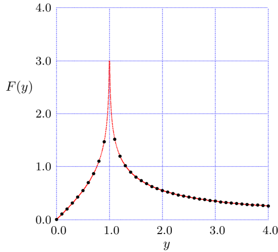
Figure A.4: F(y) = \int_0^\infty [\sin(x)/x] \sin(xy) dx .
