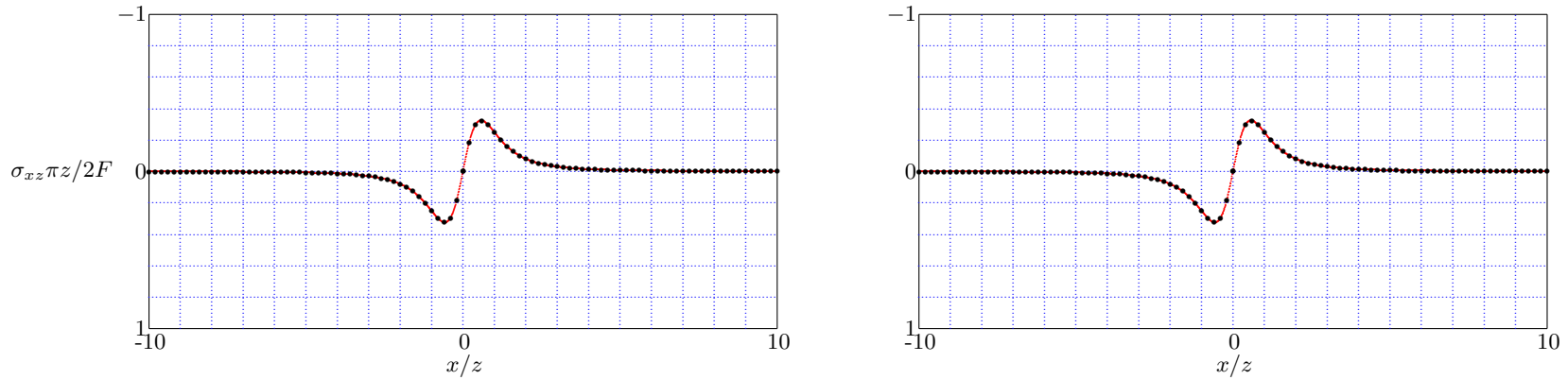
Figure 11.29: Line Load - Shear Stress, c_s t/z = 40 , \nu = 0 (left), \nu = 0.5 (right).
