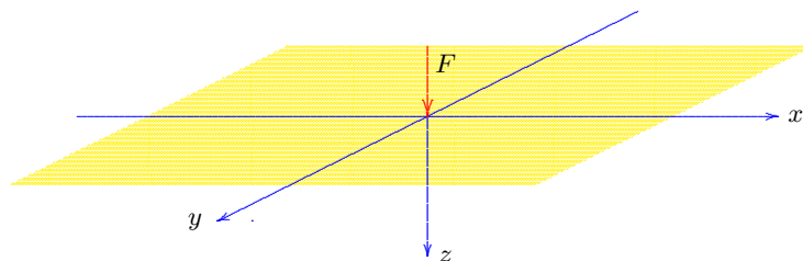
Figure 13.1: Point load on half space.
