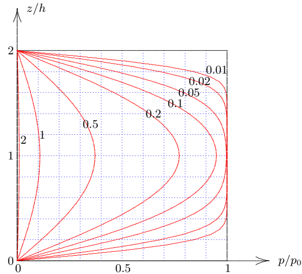
Figure 4.6: Analytical solution of Terzaghi's problem.
