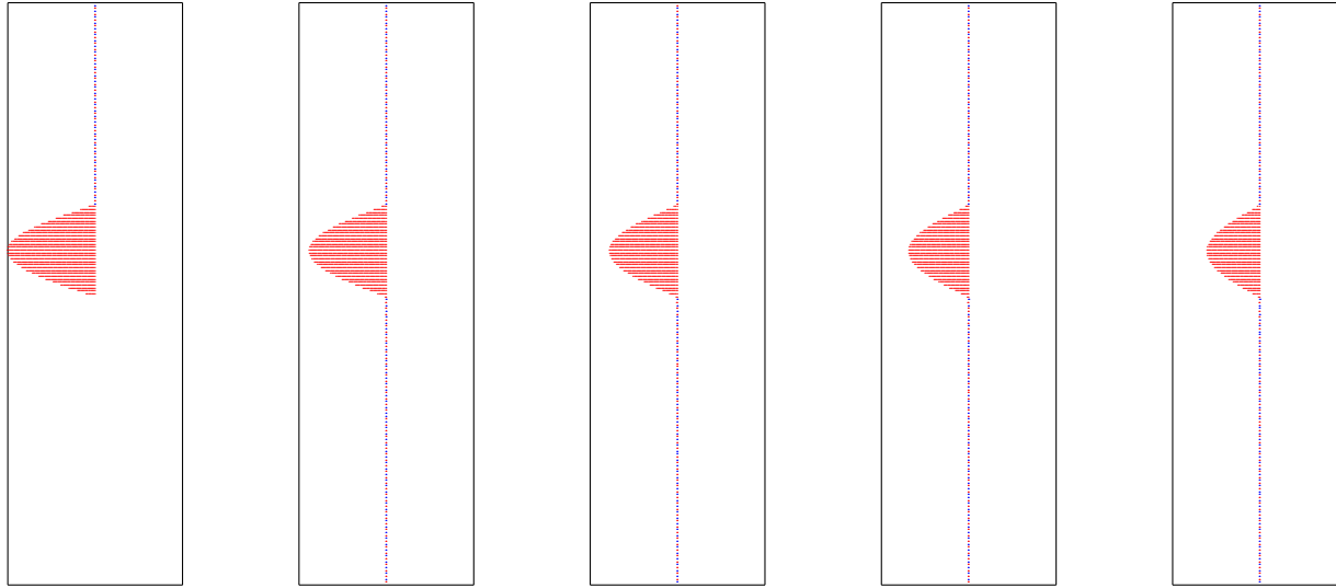
Figure 2.14: Block wave in pile, with friction.
