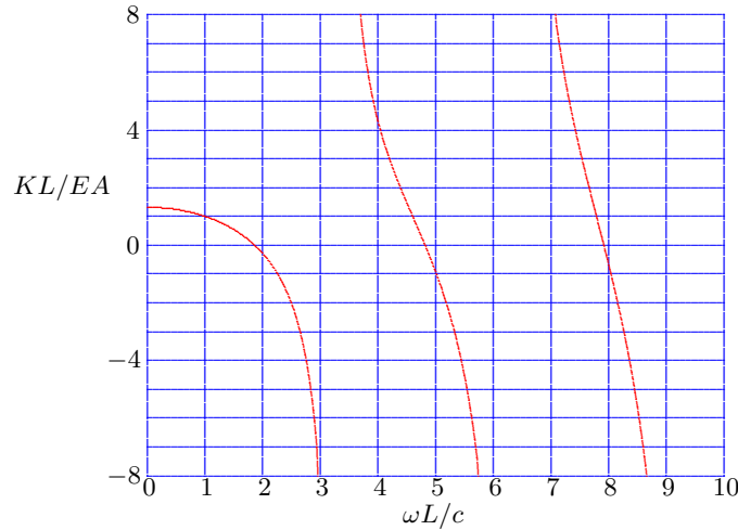
Figure 2.11: Spring constant ( H/L = 1 ).
