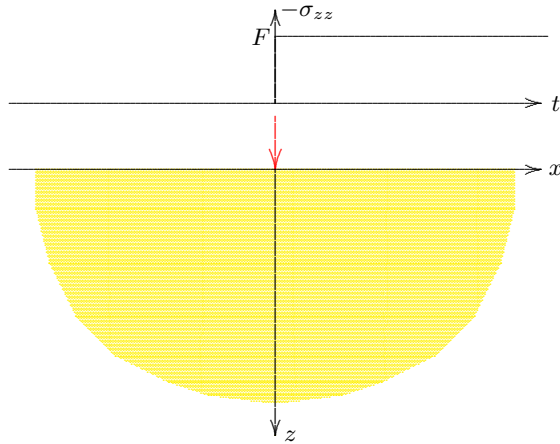
Figure 11.17: Half plane with line load.
