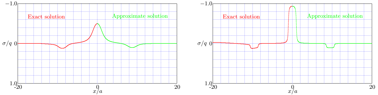
Figure 12.12: Strip Load - Isotropic Stress, c_s t/a = 10 ; \nu = 0 , z/a = 1 (left) and \nu = 0.5 , z/a = 0.1 .
