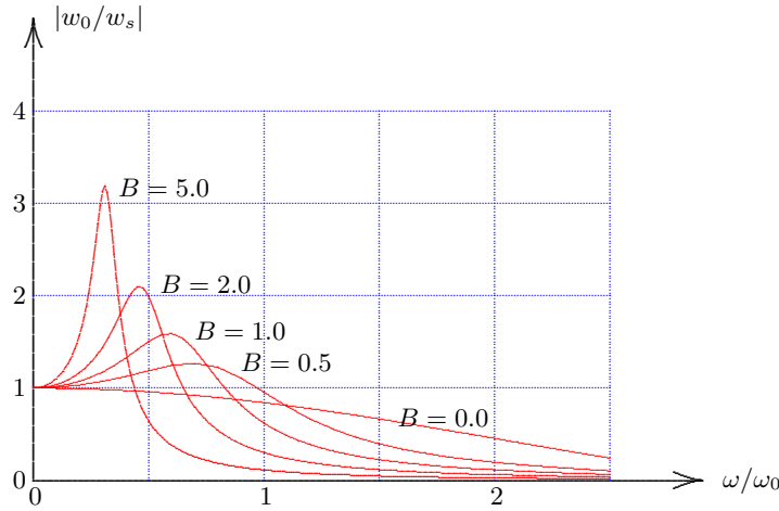
Figure 15.2: Dynamic response of footing, \nu = 1/3 .
