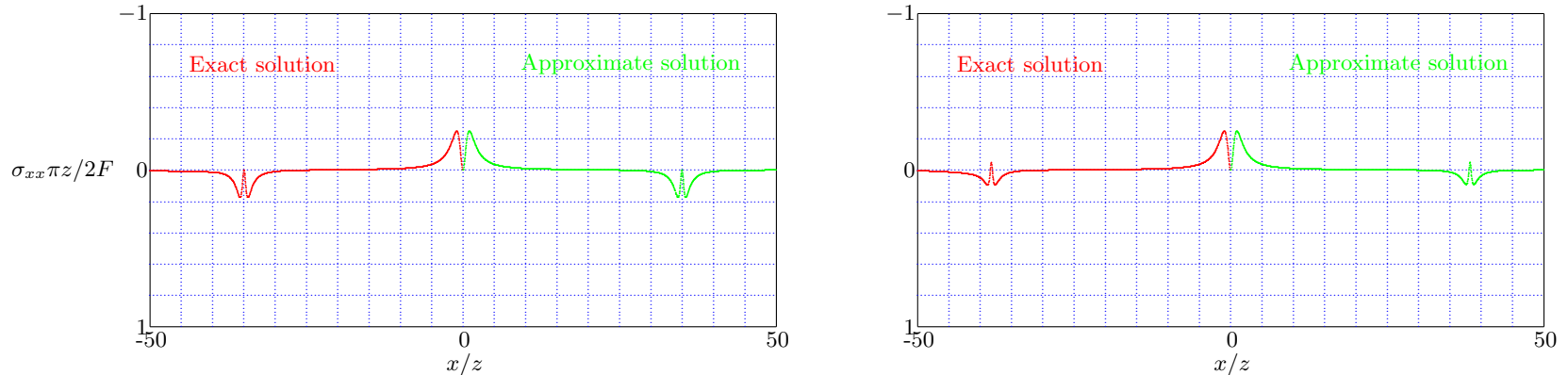
Figure 11.27: Line Load - Horizontal Normal Stress, c_s t/z = 40 , \nu = 0 and \nu = 0.5 .
