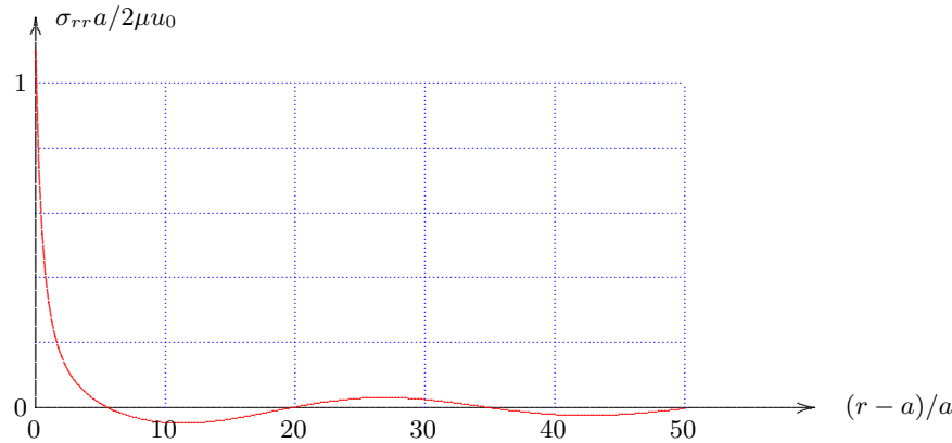
Figure 6.8: Radial stress, \omega a/c = 0.2 , \omega t/\pi = 0.5 , \nu = 0.25 .
