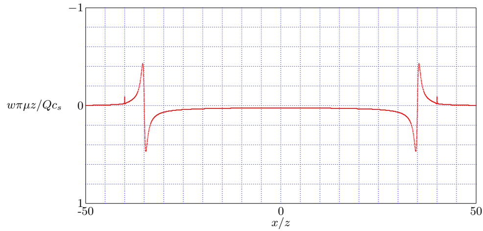
Figure 11.5: Line Pulse - Vertical Displacement, \nu = 0 , c_s t / z = 40 .
