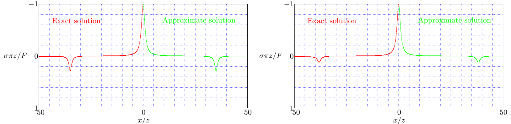
Figure 11.21: Line Load - Isotropic Stress, \nu = 0 , c_s t/z = 40 and \nu = 0.5 , c_s t/z = 40 .
