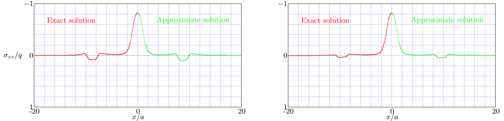
Figure 12.14: Strip Load - Vertical Normal Stress, z/a = 1 , c_s t/a = 10 ; \nu = 0 (left) and \nu = 0.5 (right).
