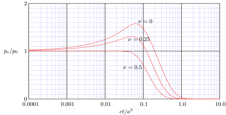
Figure 4.4: Pore pressure in the center.
