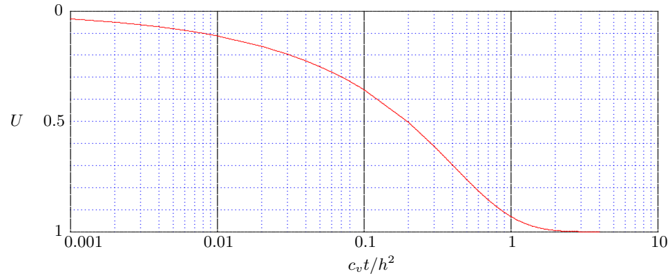
Figure 4.7: Degree of consolidation.
