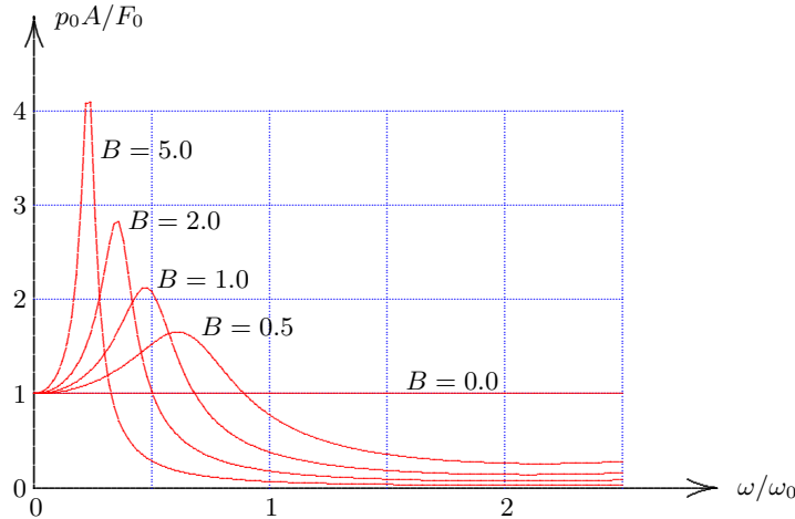
Figure 15.3: Force transmitted to half space, \nu = 1/3 .
