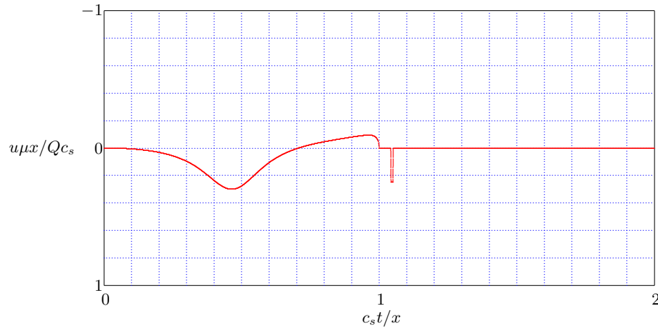
Figure 11.16: Horizontal displacement, \nu = 0.50 .
