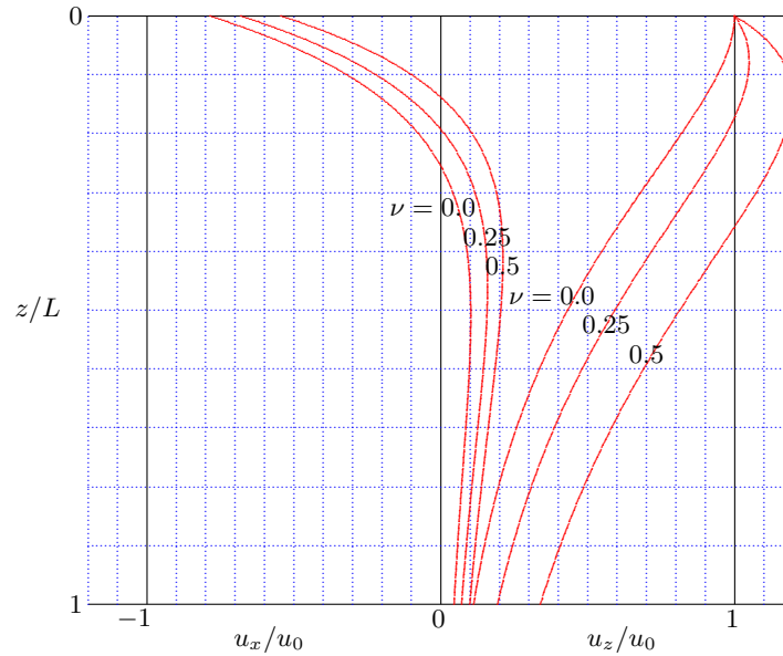
Figure 9.3: Displacements for Rayleigh wave.
