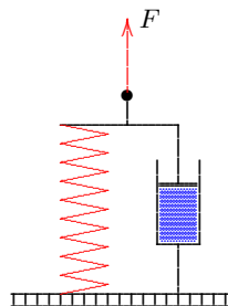
Figure 1.1: Mass supported by spring and damper.
