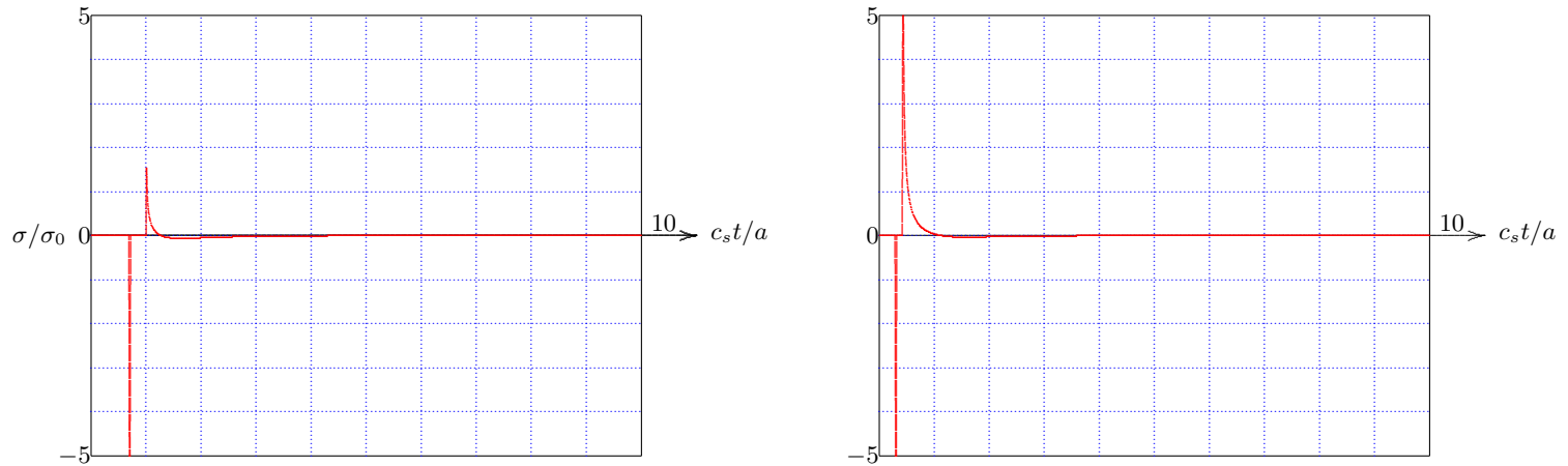
Figure 12.4: Strip Pulse - Isotropic Stress, x/a = 0 , z/a = 1 ; \nu = 0 (left) and \nu = 0.45 (right).
