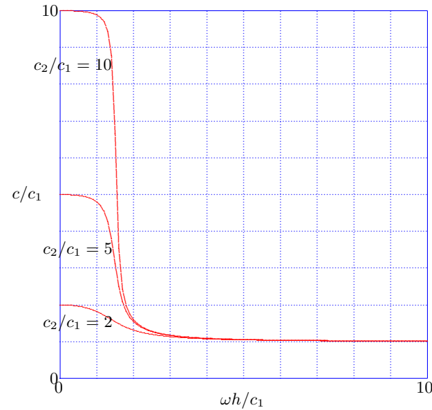
Figure 9.6: Velocity of Love wave.
