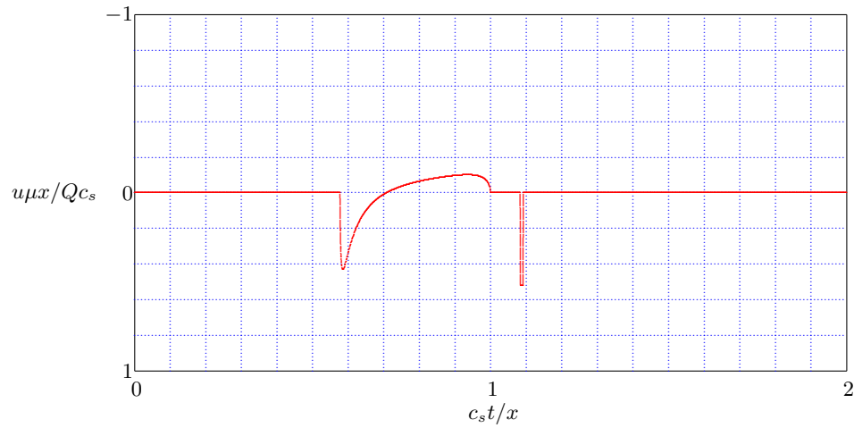
Figure 11.15: Horizontal displacement, \nu = 0.25 .
