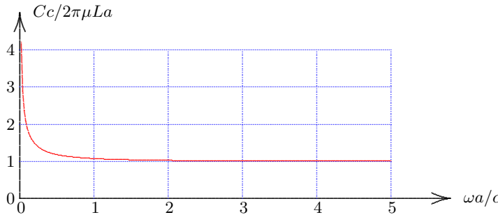
Figure 6.17: Equivalent damping.
