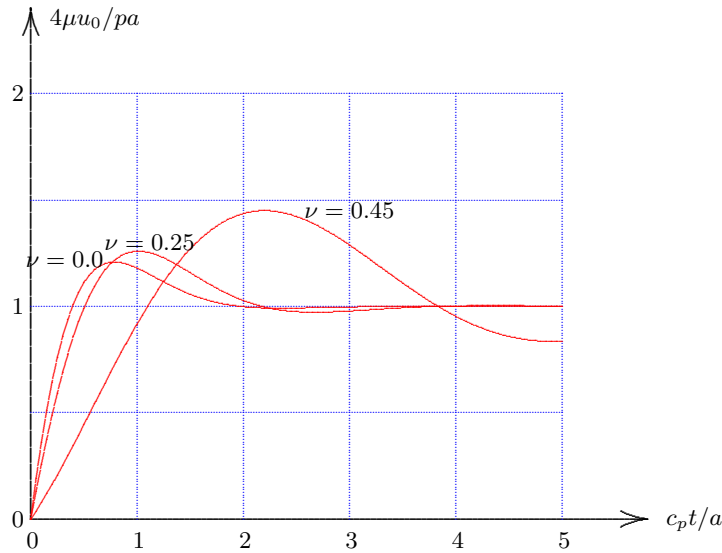
Figure 7.8: Displacement of boundary.
