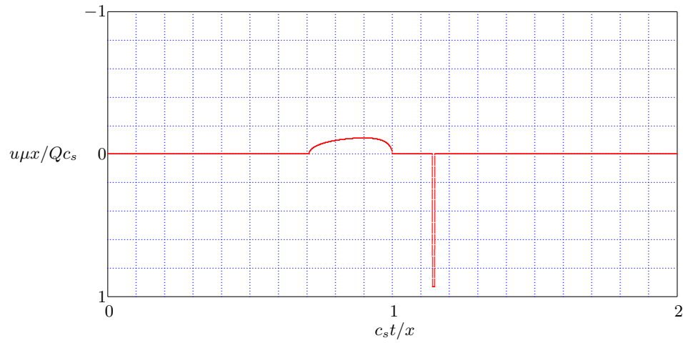
Figure 11.14: Horizontal displacement, \nu = 0.00 .
