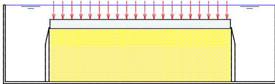
Figure 4.5: Terzaghi's problem.
