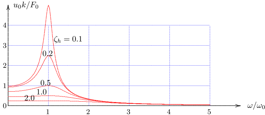
Figure 1.7: Amplitude of forced vibration, hysteretic damping.
