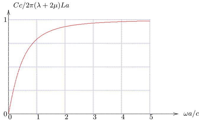
Figure 6.11: Equivalent Damping.
