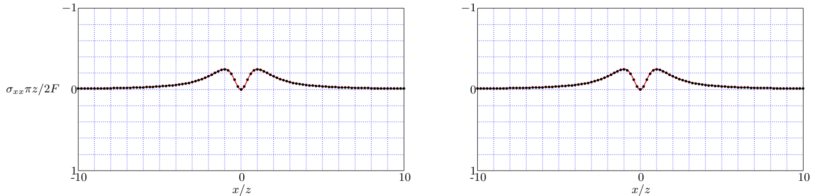
Figure 11.26: Line Load - Horizontal Normal Stress, c_s t/z = 40 , \nu = 0 (left), \nu = 0.5 (right).
