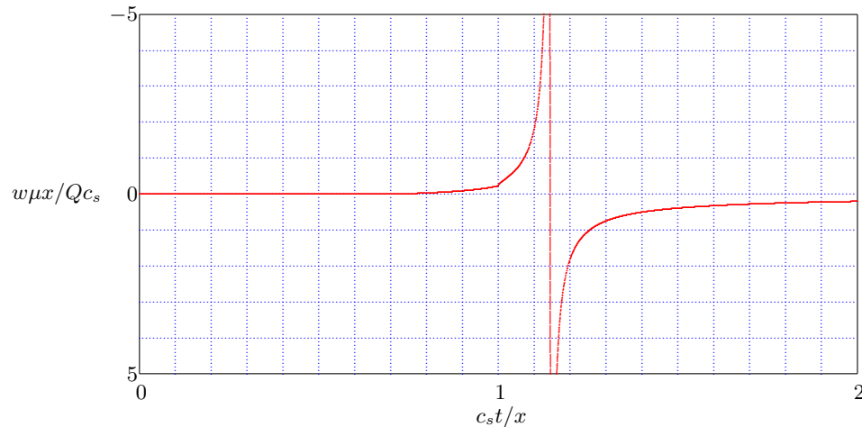
Figure 11.7: Vertical displacement, \nu = 0.00 .
