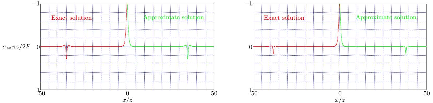
Figure 11.24: Line Load - Vertical Normal Stress, c_s t/z = 40 , \nu = 0 and \nu = 0.5 .
