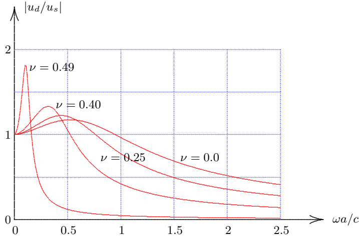
Figure 6.9: Dynamic amplification factor.
