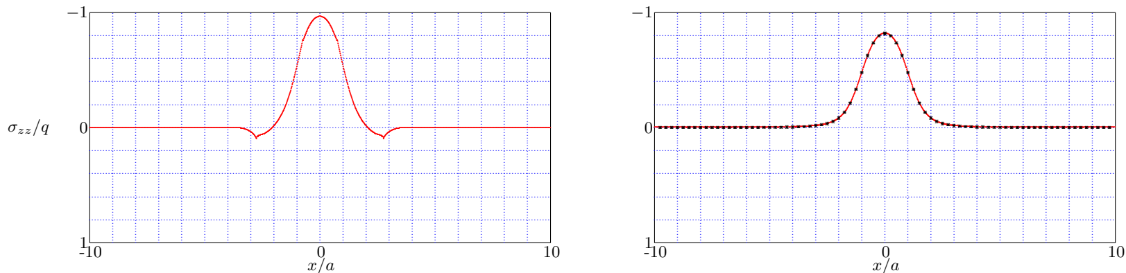
Figure 12.13: Strip Load - Vertical Normal Stress, \nu = 0.0 , z/a = 1 ; c_s t/a = 2 (left) and c_s t/a = 20 (right).
