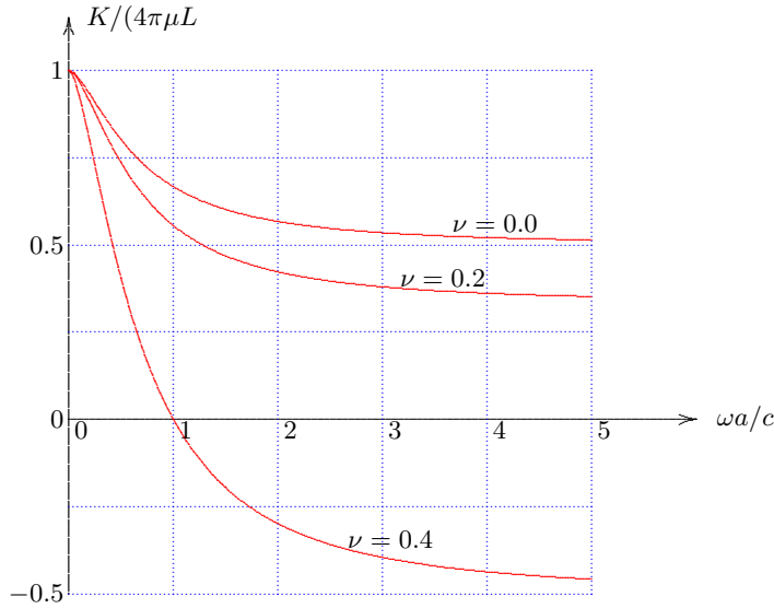
Figure 6.10: Equivalent spring.
