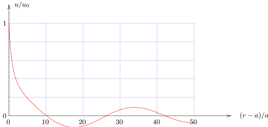
Figure 6.7: Radial displacement, \omega a/c = 0.2 , \omega t/\pi = 0.5 .
