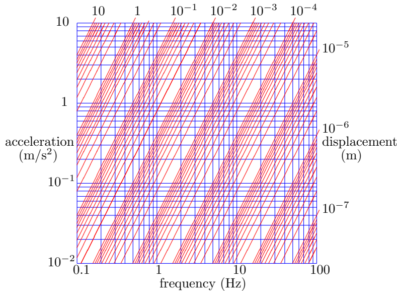
Figure 15.5: Frequency, displacement and acceleration.
