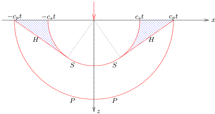
Figure 11.6: The three wave fronts.
