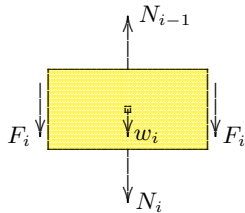
Figure 2.12: Element of pile.
