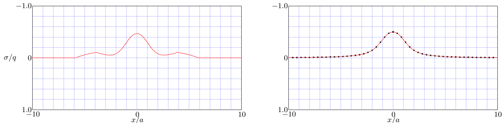
Figure 12.9: Strip Load - Isotropic Stress, \nu = 0.4 , z/a = 1 ; c_s t/a = 2 (left) and c_s t/a = 20 (right).
