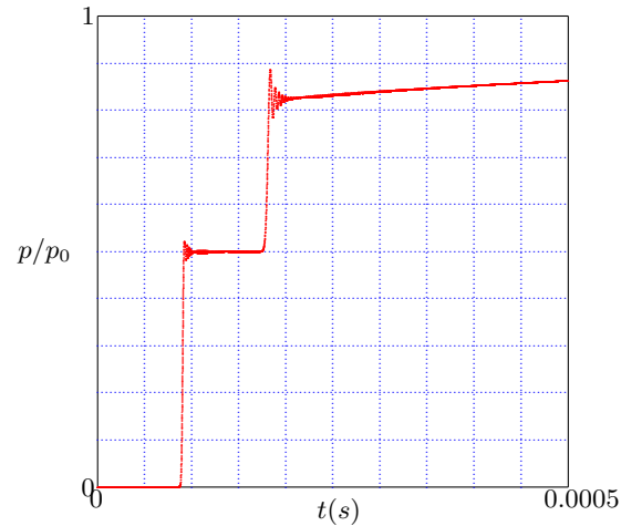
Figure 5.4: Shock wave in porous medium - Numerical solution.
