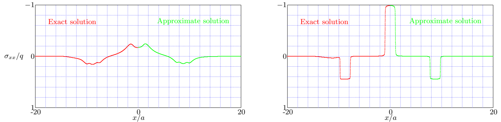
Figure 12.16: Strip Load - Horizontal Normal Stress, \nu = 0 , c_s t/a = 10 ; z/a = 1 (left) and z/a = 0.01 (right).
