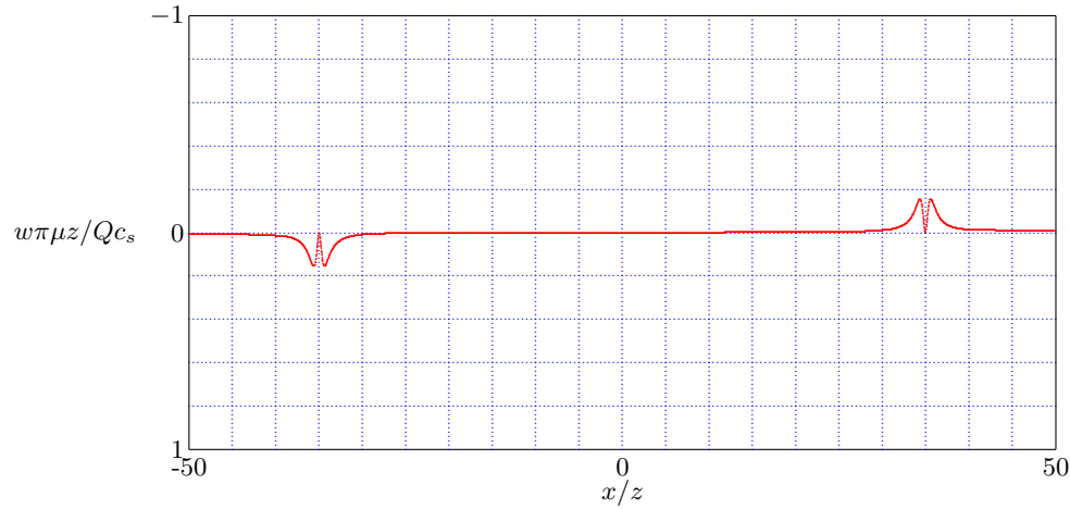
Figure 11.12: Line Pulse - Horizontal Displacement, \nu = 0 , c_s t/z = 40 .
