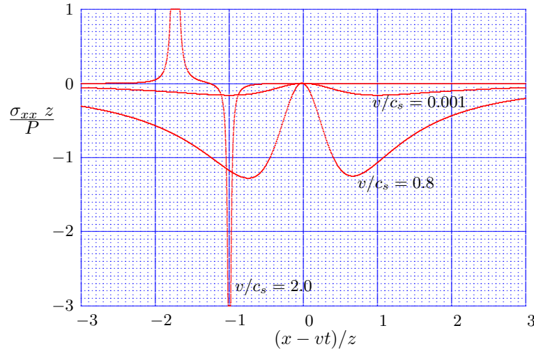
Figure 14.9: Moving point load, horizontal normal stress, \nu = 0.0 , \zeta = 0.01 .
