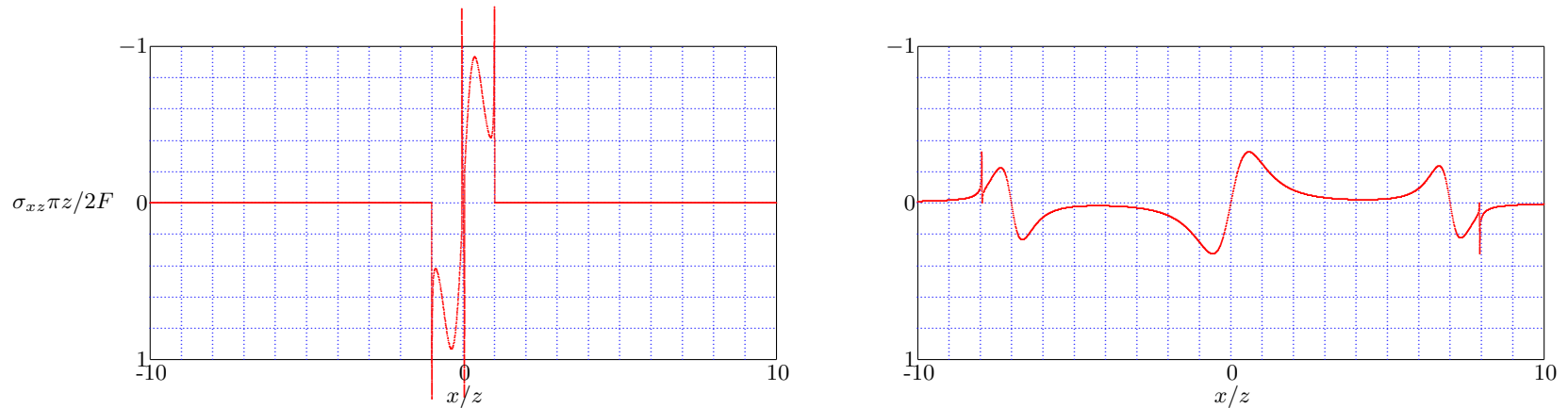
Figure 11.28: Line Load - Shear Stress, \nu = 0 , c_s t/z = 1 , (left) and c_s t/z = 8 .
