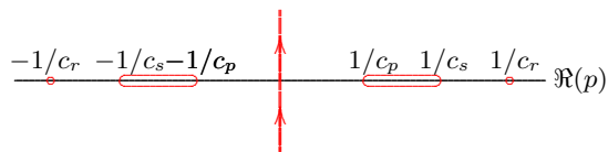
Figure 11.10: Branch cuts in the p -plane.
