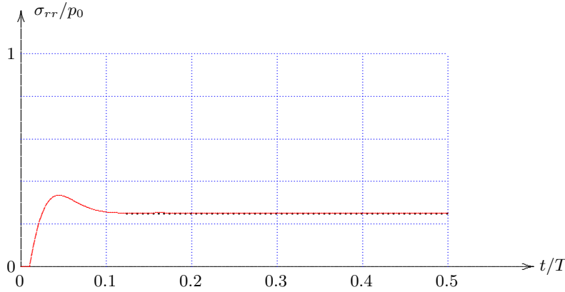
Figure 6.14: Radial stress, cT/a = 100 , \nu = 0.25 , r/a = 2 .
