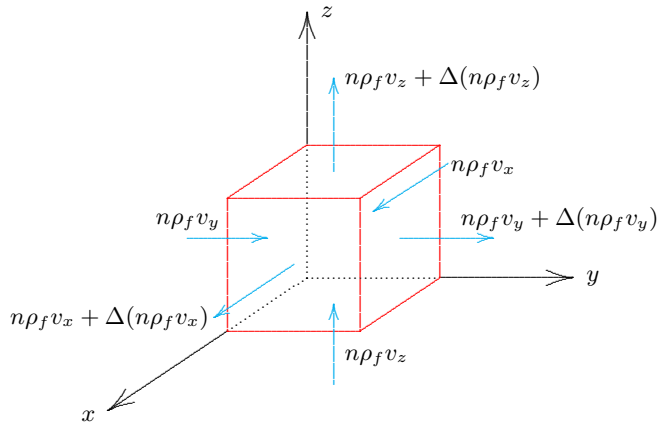
Figure 4.1: Conservation of mass of the fluid.
