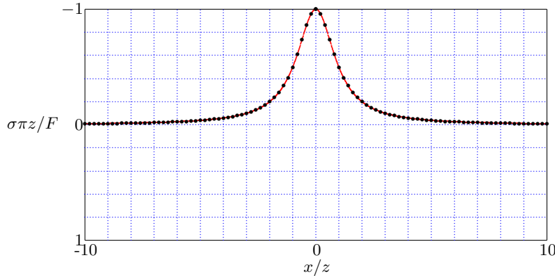
Figure 11.19: Line Load - Isotropic Stress, \nu = 0 , c_s t/z = 20 and \nu = 0.5 , c_s t/z = 20 .
