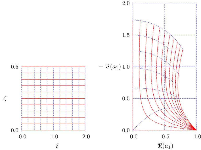
Figure 14.1: First root a_1 as a function of \xi and \zeta , for small values of \zeta .
