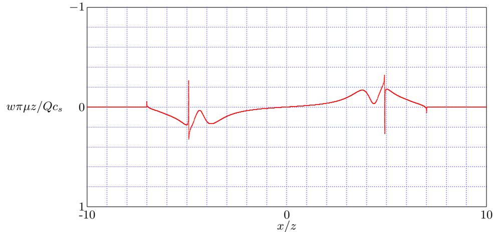
Figure 11.11: Line Pulse - Horizontal Displacement, \nu = 0 , c_s t/z = 5 .
