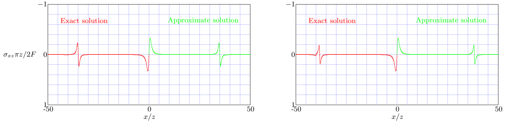
Figure 11.30: Line Load - Shear Stress, c_s t/z = 40 , \nu = 0 and \nu = 0.5 .
