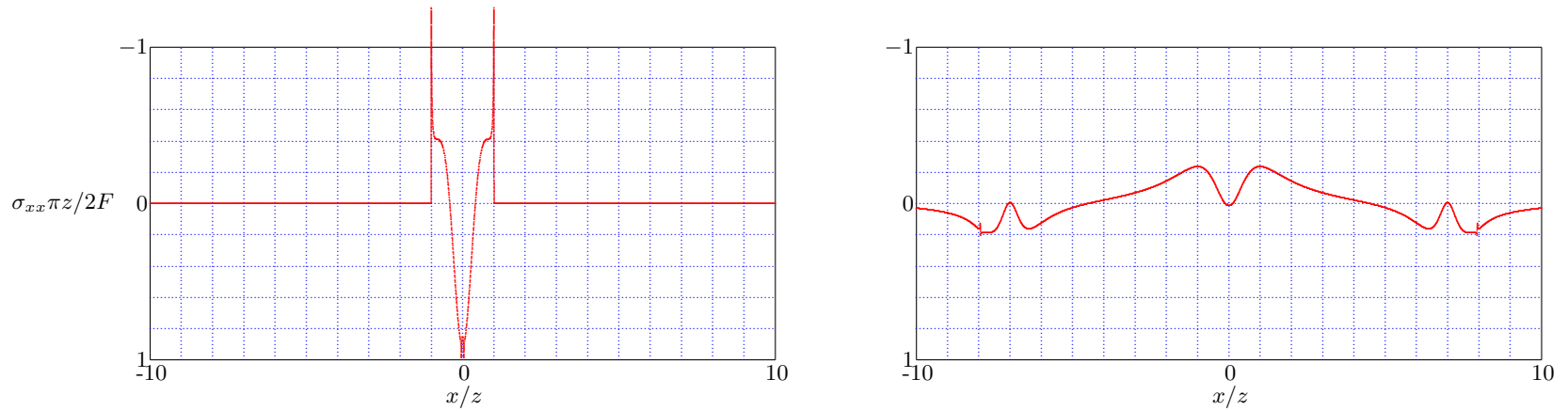
Figure 11.25: Line Load - Horizontal Normal Stress, \nu = 0 , c_s t/z = 1 (left) and c_s t/z = 8 .
