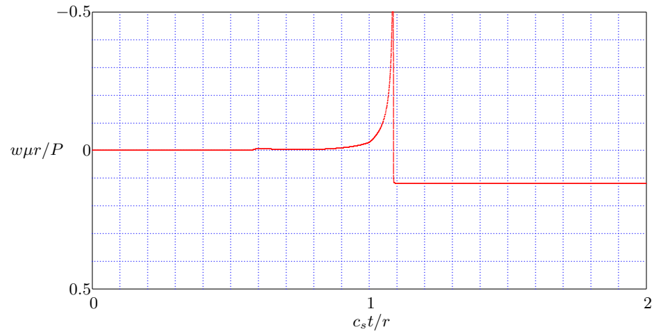
Figure 13.5: Vertical displacement, \nu = 0.25 .
