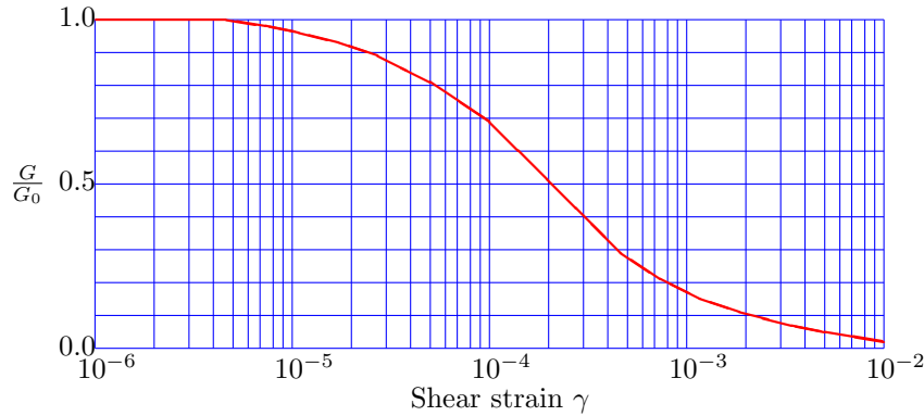
Figure 15.4: Dynamic shear modulus.
