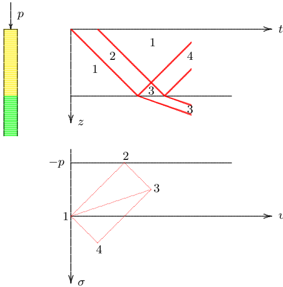
Figure 2.9: Graphical solution using characteristics.
