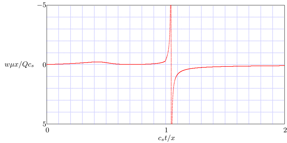
Figure 11.9: Vertical displacement, \nu = 0.50 .
