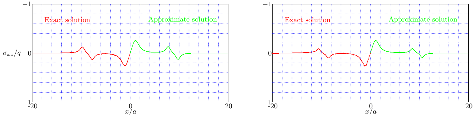
Figure 12.19: Strip Load - Shear Stress, z/a = 1 , c_s t/a = 10 ; \nu = 0 (left) and \nu = 0.5 (Right).
