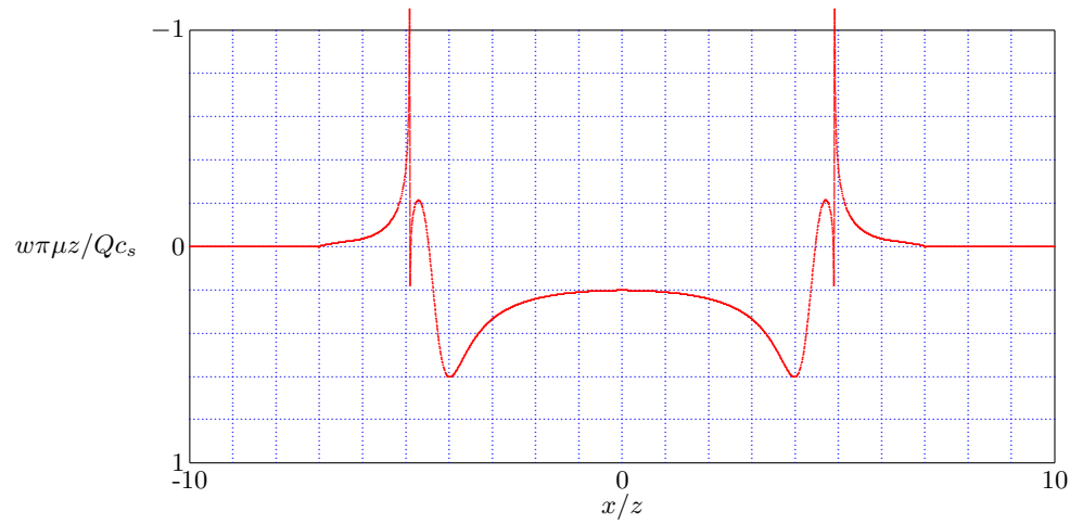
Figure 11.4: Line Pulse - Vertical Displacement, \nu = 0 , c_s t / z = 5 .
