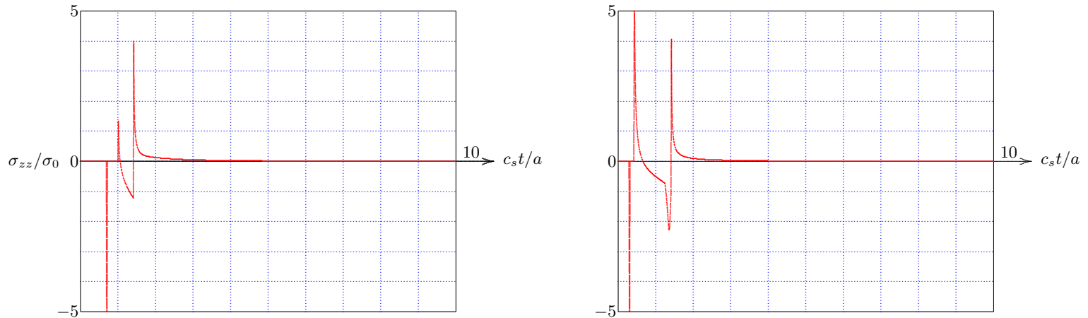
Figure 12.5: Strip Pulse - Vertical Normal Stress, x/a = 0 , z/a = 1 ; \nu = 0 (left) and \nu = 0.45 (right).
