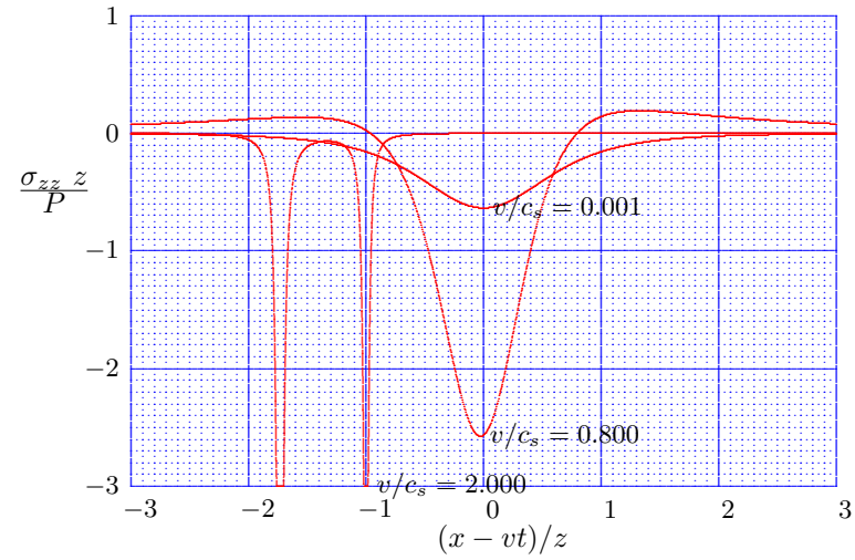
Figure 14.5: Moving point load, vertical normal stress, \nu = 0.0 , \zeta = 0.01 .
