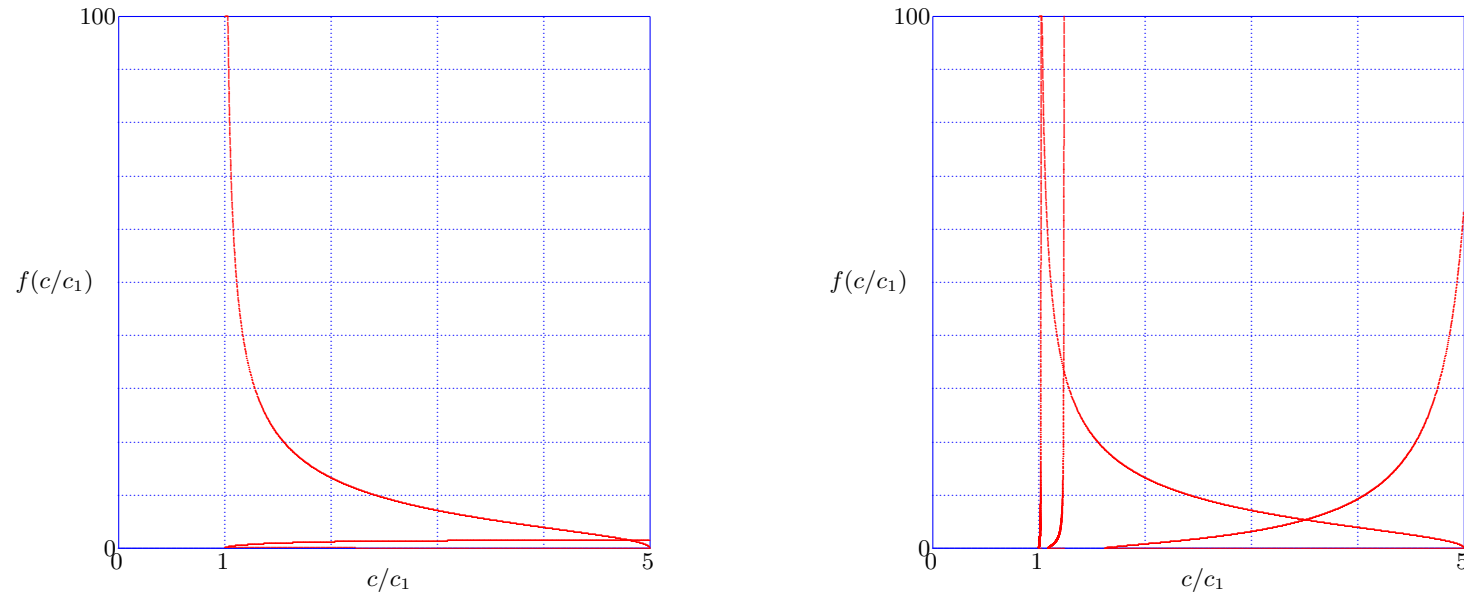
Figure 9.5: Determination of the velocity of a Love wave, c_2/c_1 = 5 ; \omega h/c_1 = 1 (left), \omega h/c_1 = 8 (right).
