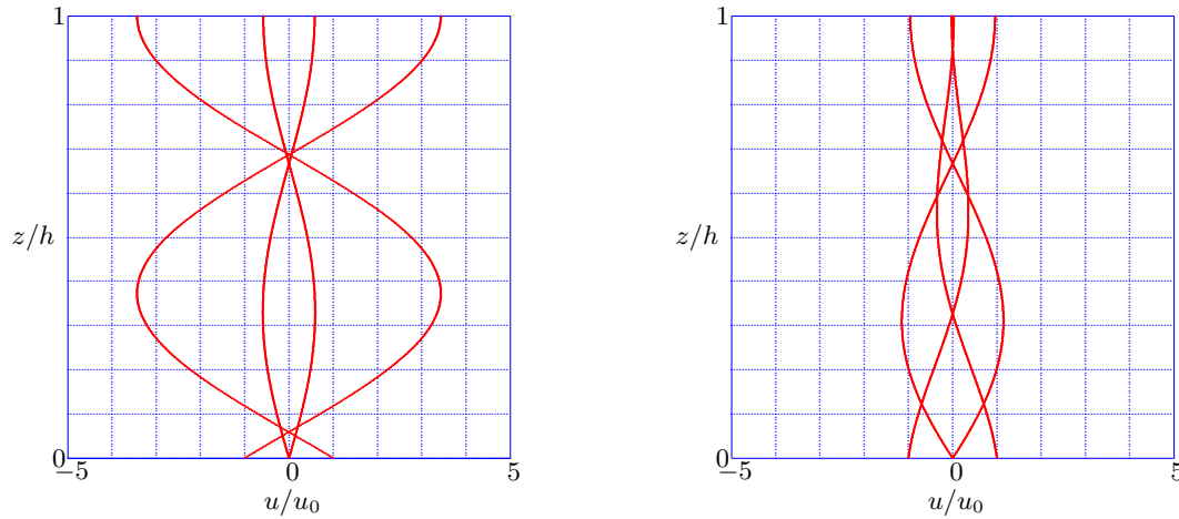
Figure 3.6: Displacements as a function of depth, \omega h/c = 5 , \zeta = 0.01 and \zeta = 0.2 .
