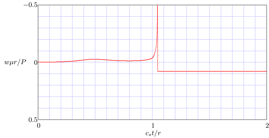
Figure 13.6: Vertical displacement, \nu = 0.50 .
