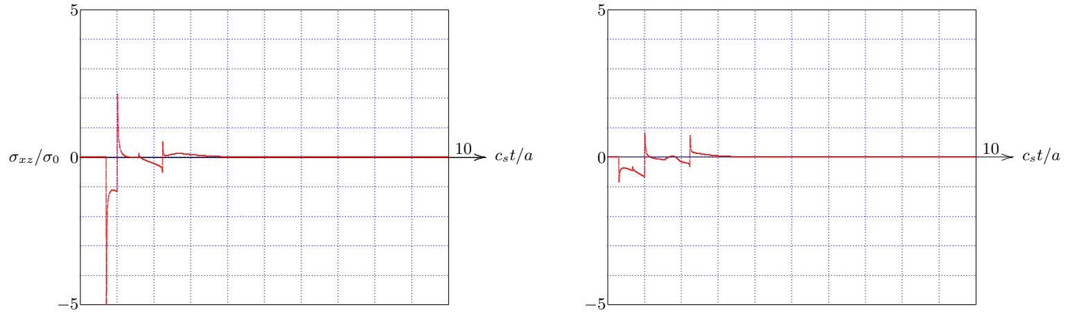
Figure 12.7: Strip Pulse - Shear Stress, x/a = 0 , z/a = 1 ; \nu = 0 (left) and \nu = 0.45 (right).
