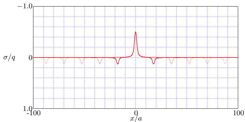
Figure 12.10: Strip Load - Isotropic Stress, \nu = 0 , z/a = 1 .
