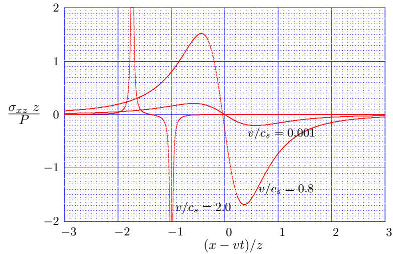
Figure 14.10: Moving point load, shear stress, \nu = 0.0 , \zeta = 0.01 .
