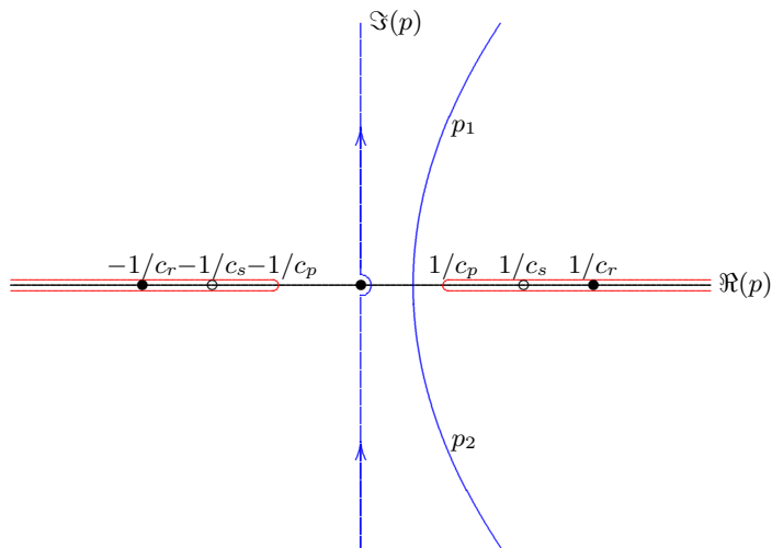
Figure 12.2: Modified integration path, for x > 0 .
