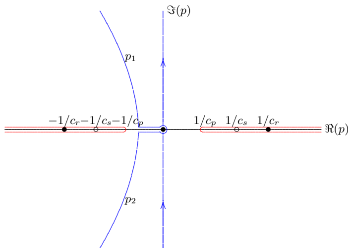
Figure 12.3: Modified integration path, if x < 0 .
