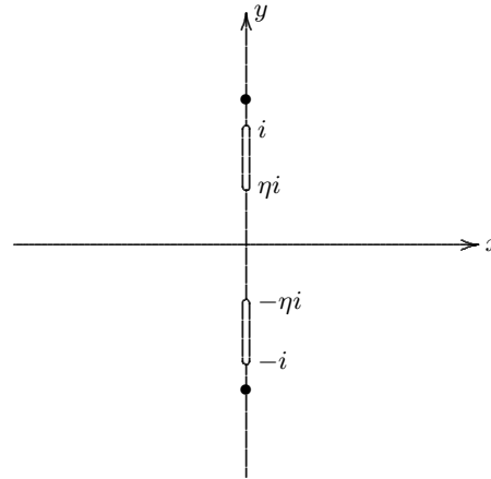
Figure 13.2: The complex z -plane.
