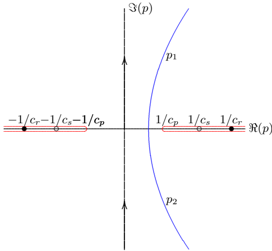
Figure 11.2: Integration path for the first integral. cut should extend towards infinity.
