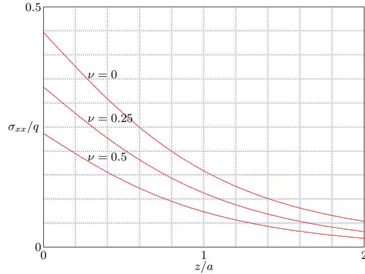
Figure 12.17: Maximum value of \sigma_{xx} in Rayleigh wave.
