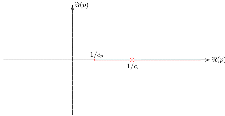
Figure 11.13: Modified integration path for z = 0 .
