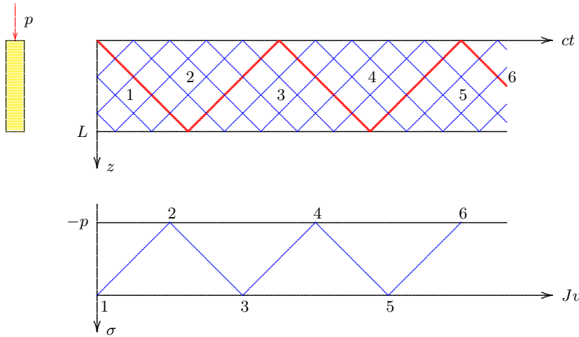
Figure 2.5: The method of characteristics.
