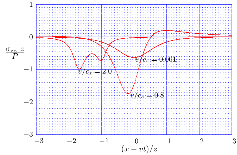
Figure 14.6: Moving point load, vertical normal stress, \nu = 0.0 , \zeta = 0.1 .
