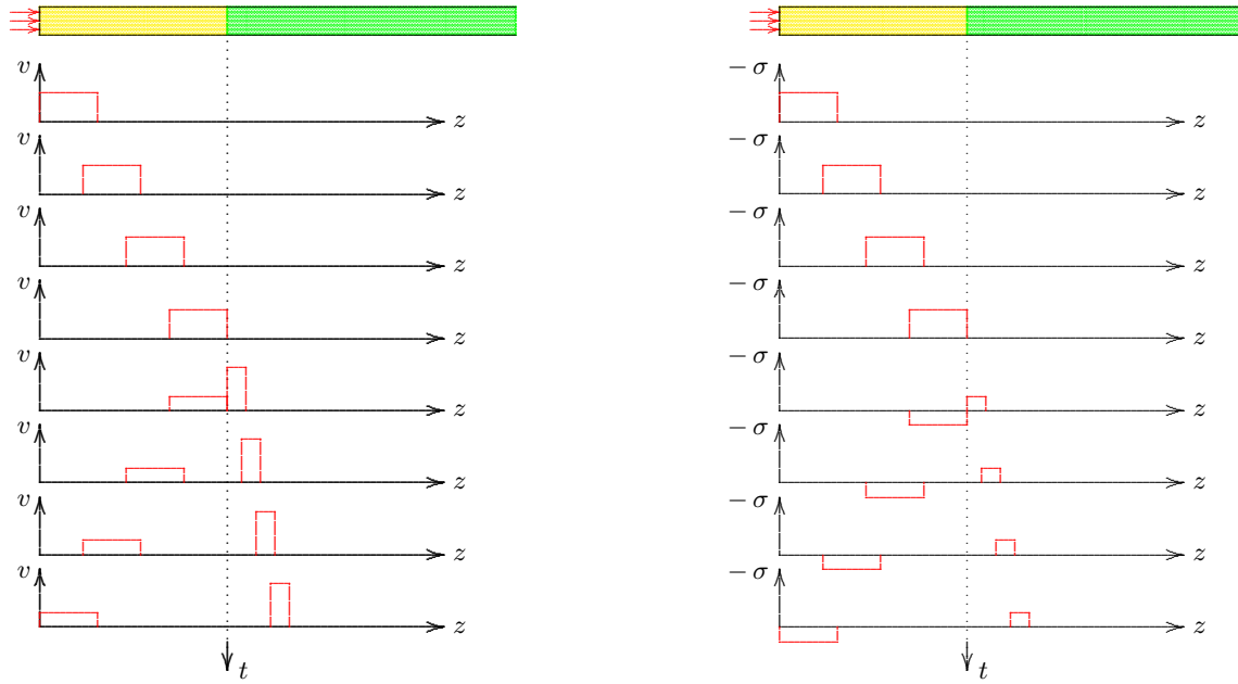
Figure 2.8: Reflection and transmission of a shock wave.
