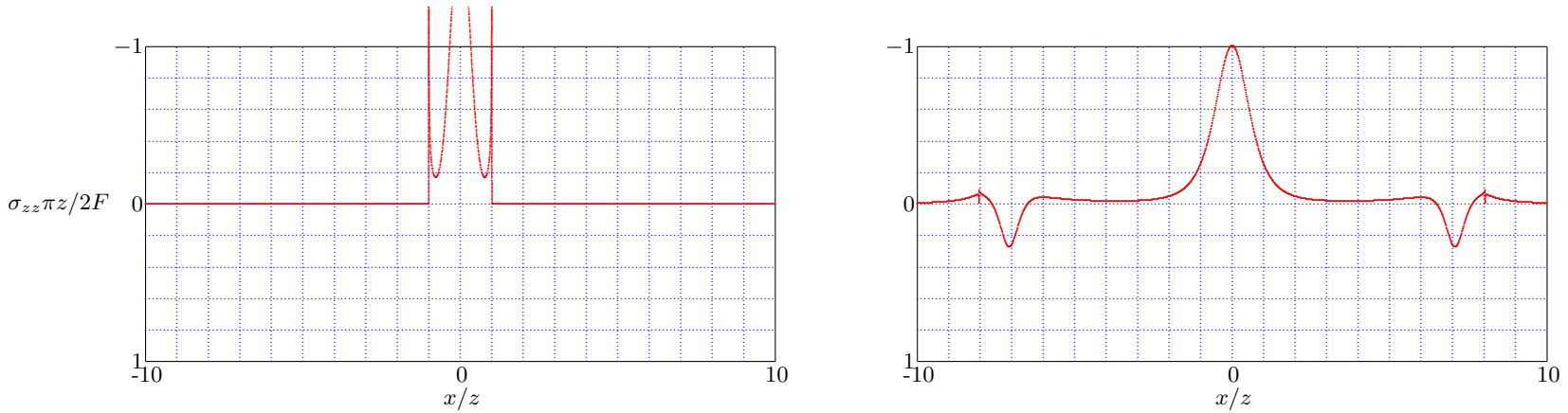
Figure 11.22: Line Load - Vertical Normal Stress, \nu = 0 , c_s t/z = 1 (left), c_s t/z = 8 (right).
