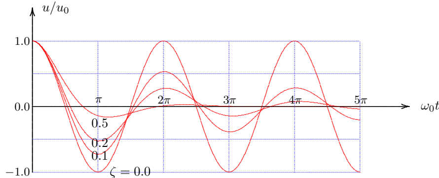
Figure 1.2: Free vibrations of a weakly damped system.
