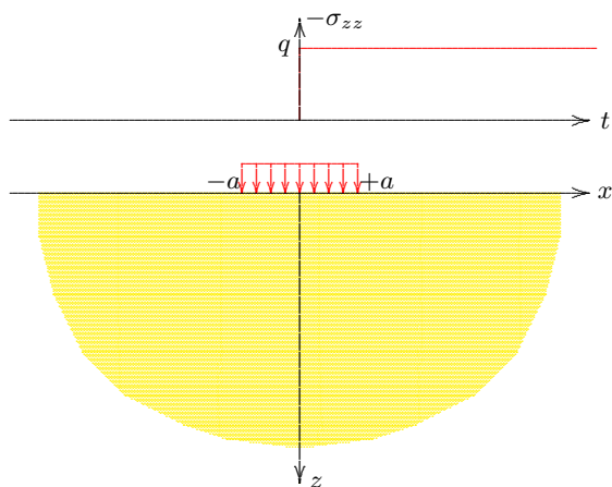
Figure 12.8: Half plane with strip load.
