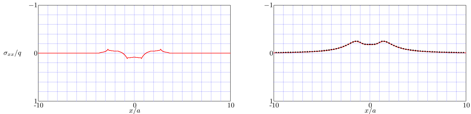
Figure 12.15: Strip Load - Horizontal Normal Stress, \nu = 0.0 , z/a = 1 ; c_s t/a = 2 (left) and c_s t/a = 20 (right).
