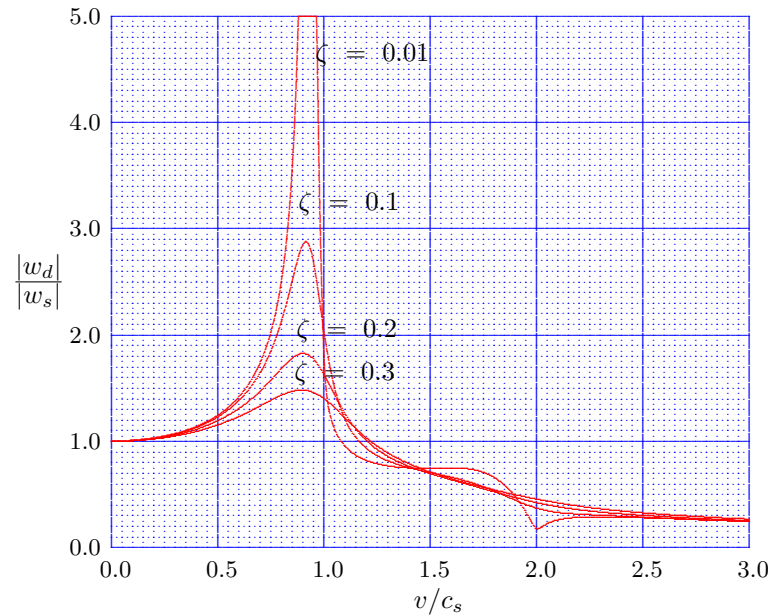
Figure 14.4: Moving strip load, Dynamic amplification factor, \nu = 0.3333 .
