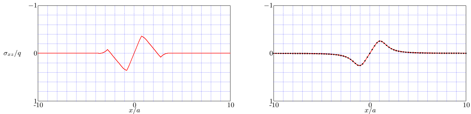
Figure 12.18: Strip Load - Shear Stress, \nu = 0.0 , z/a = 1 ; c_s t/a = 2 (left) and c_s t/a = 20 (right).
