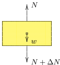
Figure 2.1: Element of pile.
