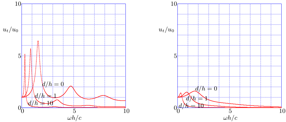
Figure 3.7: Amplitude of wave at the top of the layer, \zeta = 0.1 and \zeta = 0.5 .
