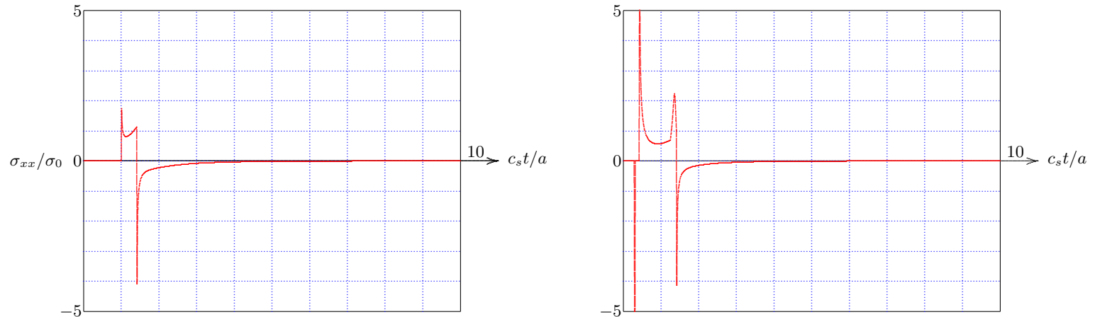
Figure 12.6: Strip Pulse - Horizontal Normal Stress, x/a = 0 , z/a = 1 ; \nu = 0 (left) and \nu = 0.45 (right).
