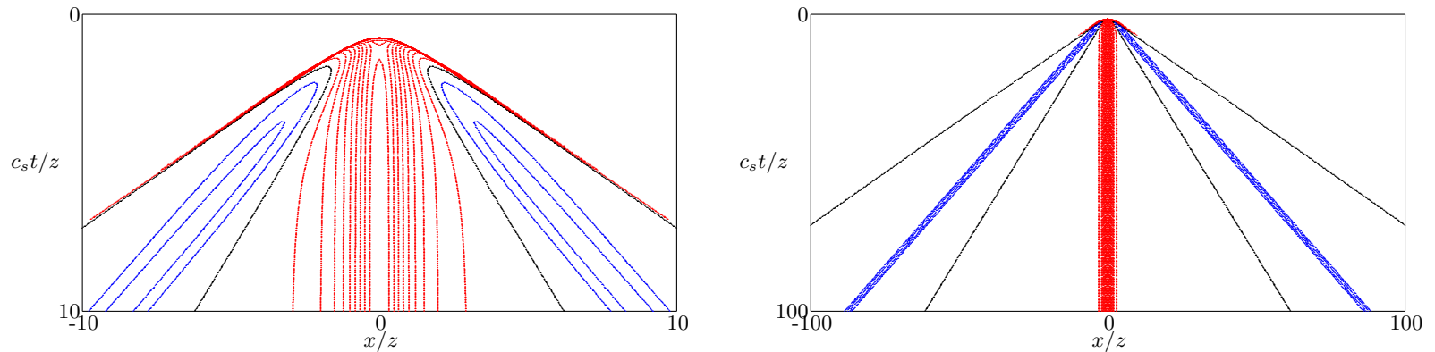
Figure 11.20: Line Load - Contours of isotropic Stress, \nu = 0 .
