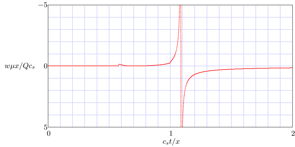
Figure 11.8: Vertical displacement, \nu = 0.25 .
