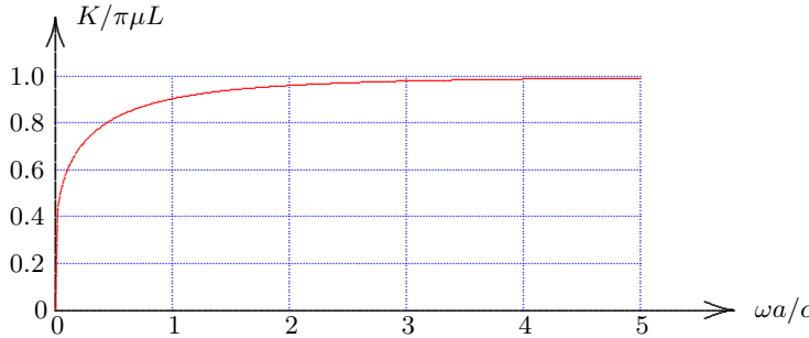
Figure 6.16: Equivalent spring.
