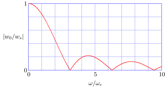
Figure 10.5: Dynamic Amplification.
