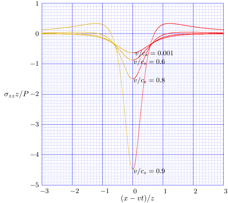
Figure 14.7: Comparison of solutions, \nu = 0.333333 .
