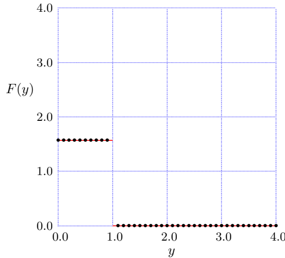
Figure A.3: F(y) = \int_0^\infty [\sin(x)/x] \cos(xy) dx .
