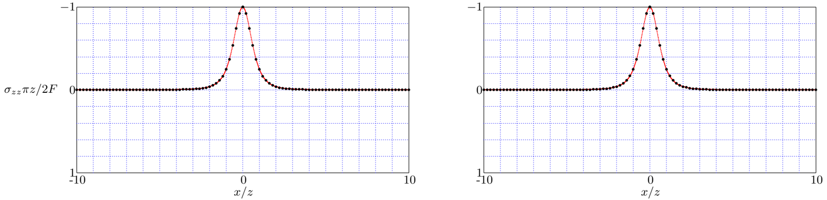
Figure 11.23: Line Load - Vertical Normal Stress, c_s t/z = 40 , \nu = 0 (left), \nu = 0.5 (right).
