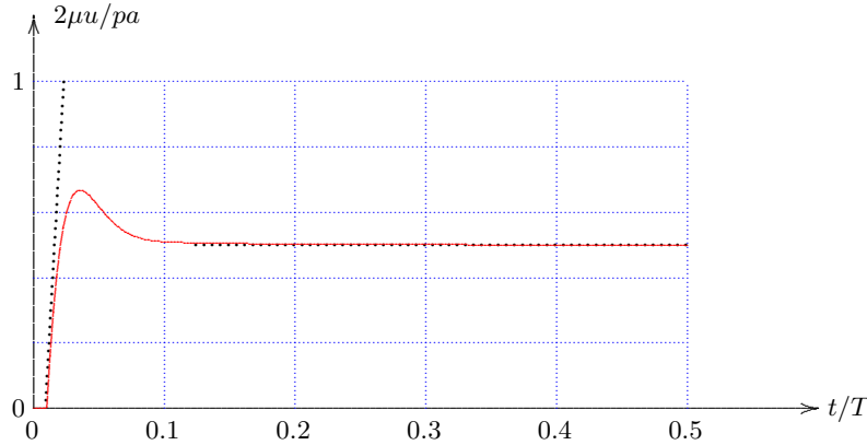
Figure 6.13: Radial displacement, cT/a = 100 , \nu = 0 , r/a = 2 .
