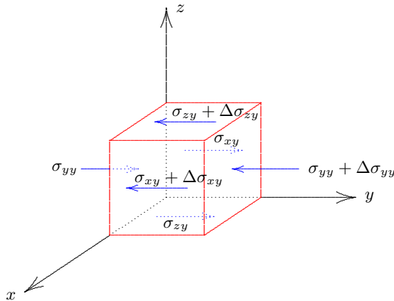
Figure 4.2: Equilibrium of element.
