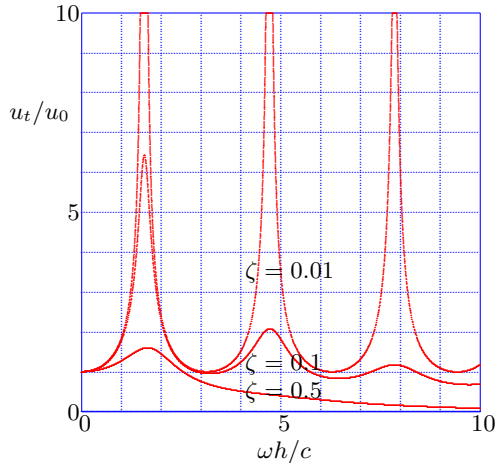
Figure 3.5: Amplitude of wave at the top of the layer.
