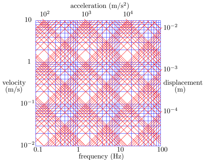
Figure 15.6: Frequency, displacement, velocity and acceleration.
