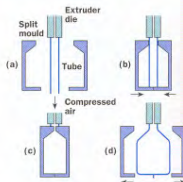
Bottle blowing
