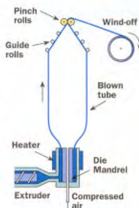
Film blowing
