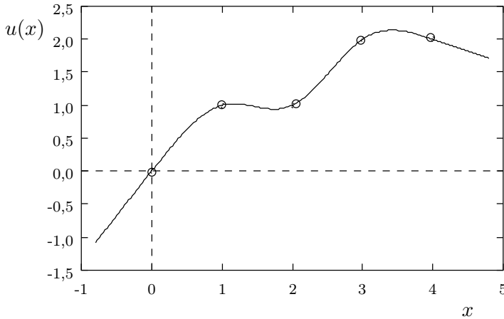
Figure 5.15 – Krigage cubique
