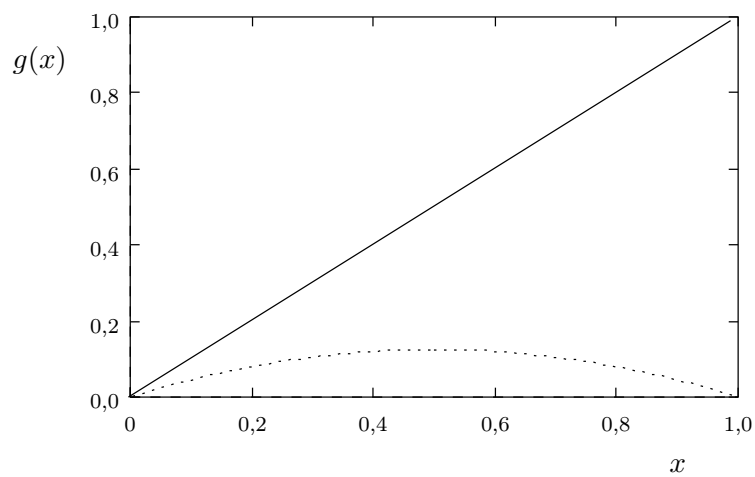
Figure 4.1 – Application quadratique : \lambda = 0,5
