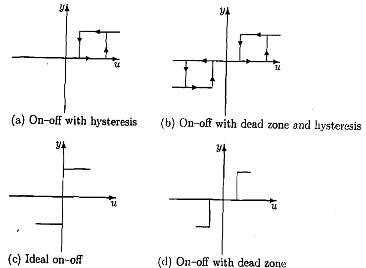
Figure 5.2: Relay characteristics
