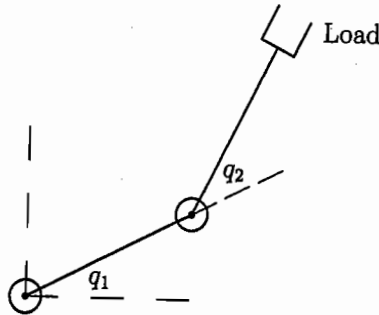
Figure 14.23: Two-link robot.
