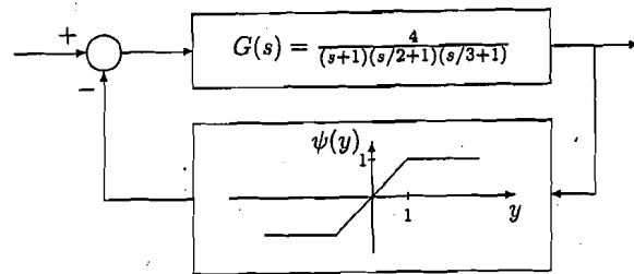
Figure 7.7: Feedback connection with saturation nonlinearity.
