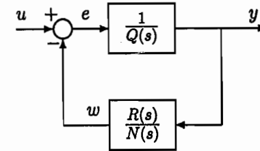
Figure 13.1: Feedback representation of H(s) .
