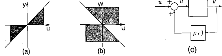
Figure 6.5: A graphical representation of u^T y \geq \delta y^T y for (a) \delta > 0 (excess of passivity); (b) \delta < 0 (shortage of passivity); (c) removal of excess or shortage of passivity by output-feedback operation.
