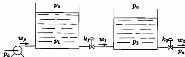
Figure 1.30: The hydraulic system of Exercise 1.21.
