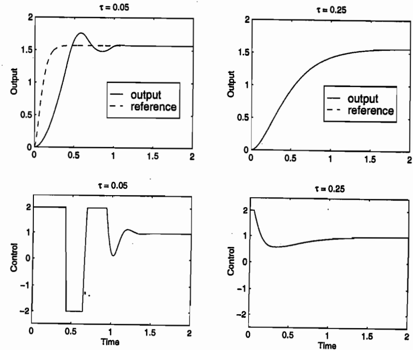
Figure 13.3: Simulation of the tracking control of Example 13.22.
