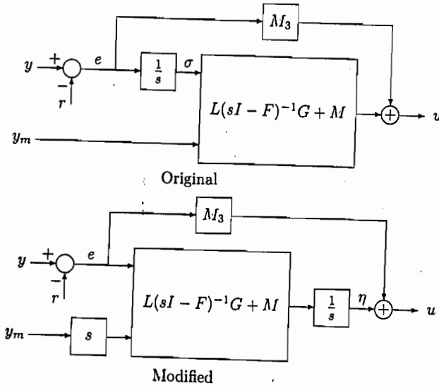
Figure 12.4: Modification of the gain-scheduled controller.
