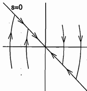
Figure 14.1: A typical phase portrait under sliding mode control.
