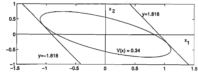
Figure 7.11: Region of attraction for Example 7.4.
