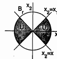
Figure 4.5: The set U for V(x) = \frac{1}{2}(x_1^2 - x_2^2) .
