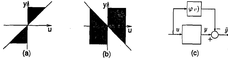
Figure 6.4: A graphical representation of u^T y \geq \epsilon u^T u for (a) \epsilon > 0 (excess of passivity); (b) \epsilon < 0 (shortage of passivity); (c) removal of excess or shortage of passivity by input-feedforward operation.
