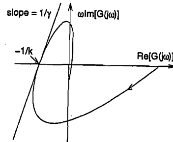
Figure 7.13: Popov plot.
