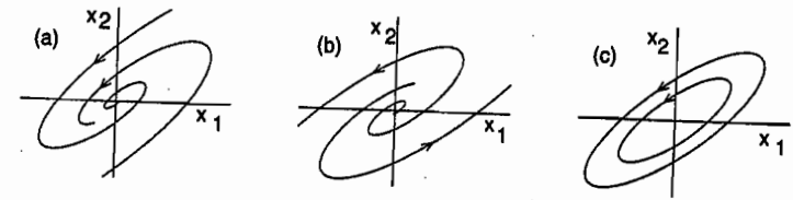
Figure 2.7: Phase portraits for (a) a stable focus; (b) an unstable focus; (c) a center.
