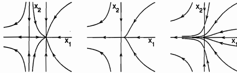
Figure 2.27: Phase portrait of the saddle-node bifurcation example for \mu > 0 (left), \mu = 0 (center), and \mu < 0 (right).
