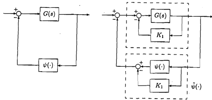
Figure 7.2: \psi \in [K_1, \infty] is transformed to \tilde{\psi} \in [0, \infty] via a loop transformation.
