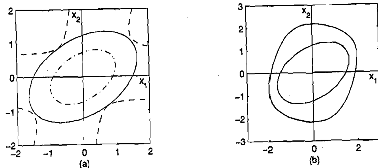
Figure 8.4: (a) Contours of \dot{V}(x) = 0 (dashed), V(x) = 0.8 (dash-dot), and V(x) = 2.25 (solid) for Example 8.9; (b) comparison of the region of attraction with its estimate.
