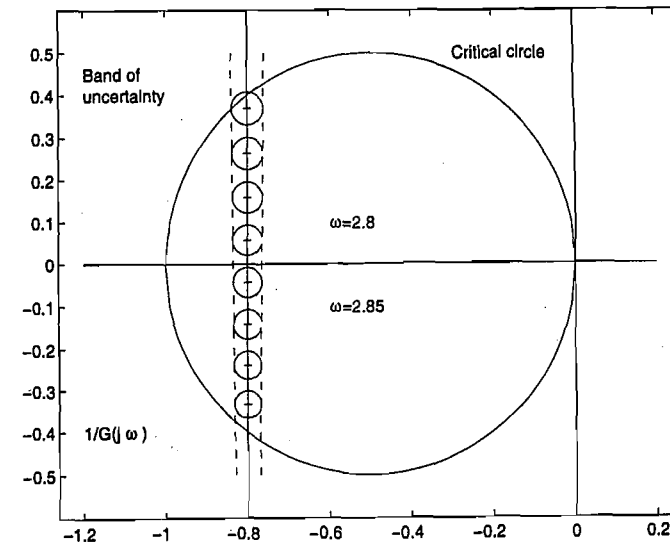
Figure 7.21: Uncertainty band for Example 7.14.
