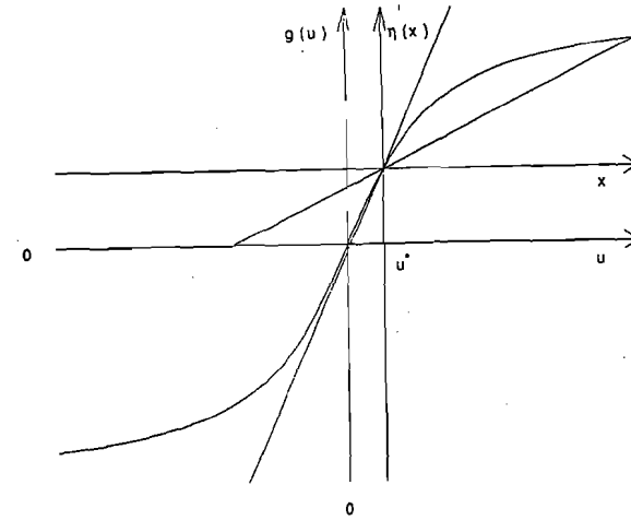
Figure 9.1: The sector nonlinearity \eta_i(x_i) of Example 9.8.
