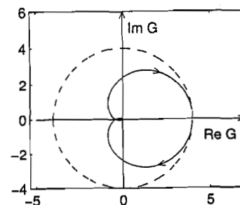
Figure 7.5: Nyquist plot for Example 7.2.
