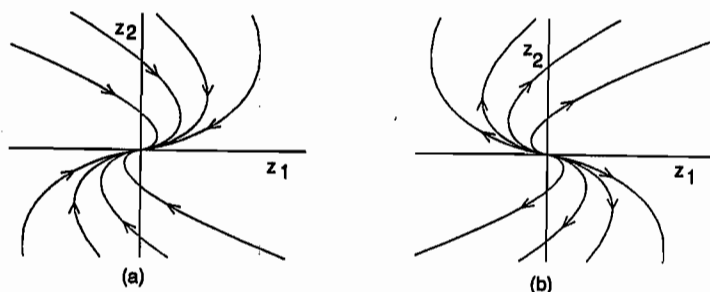
Figure 2.9: Phase portraits for the case of nonzero multiple eigenvalues when k = 1 : (a) \lambda < 0 ; (b) \lambda > 0 .
