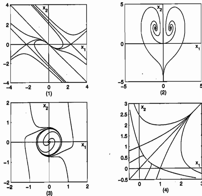
Figure 2.33: Phase portraits of Exercise 2.4.
