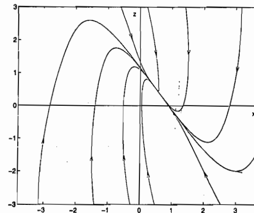
Figure 11.9: Phase portrait of Example 11.10 for \varepsilon = 0.1 .
