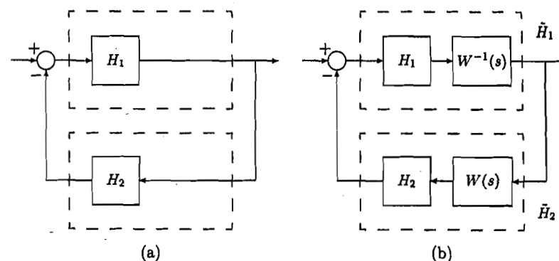
Figure 6.14: Loop transformation with dynamic multipliers.
