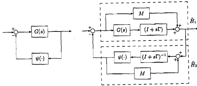
Figure 7.12: Loop transformation.
