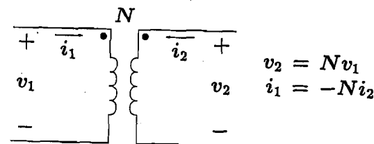
Figure 6.3: Ideal transformer
