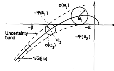
Figure 7.20: A complete intersection.
