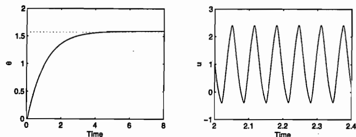
Figure 14.6: Modified sliding mode control with unmodeled actuator dynamics.
