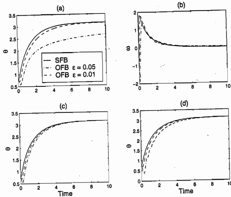
Figure 14.22: Comparison of state feedback (SFB) and output feedback (OFB) for Example 14.19. Figures (a) and (b) show \theta and \omega = \dot{\theta} for a nonlinear high-gain observer with nominal m and \ell . Figure (c) shows \theta for a nonlinear high-gain observer with actual m and \ell . Figure (d) shows \theta for a linear high-gain observer.
