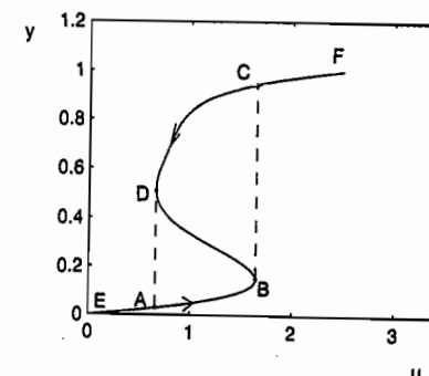
Figure 2.15: Hysteresis characteristics of the tunnel-diode circuit.
