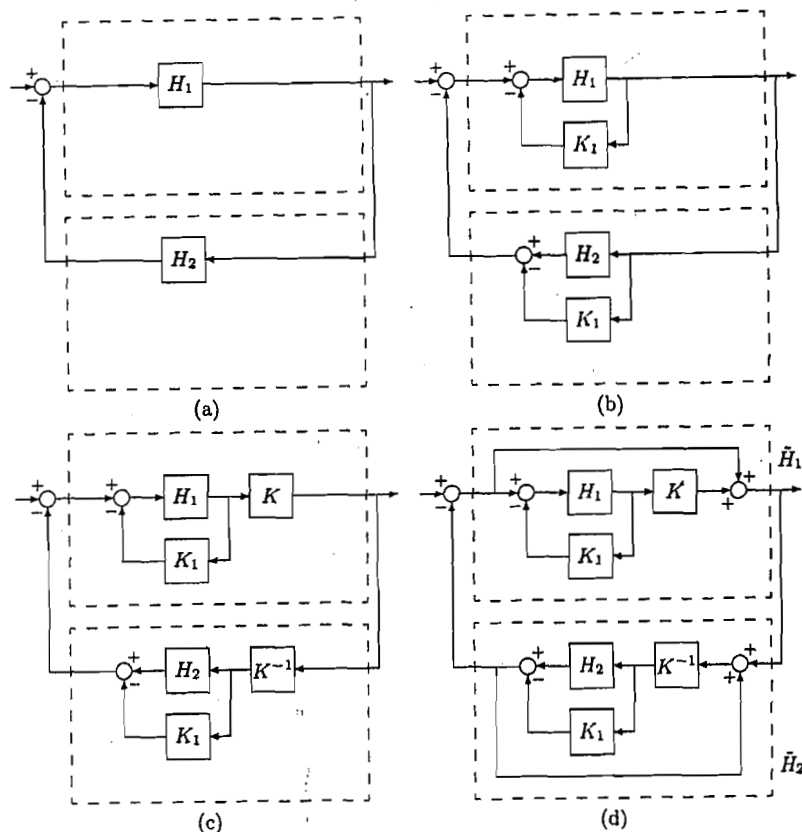
Figure 6.13: Loop transformation with constant gains. A memoryless function H_2 in the sector [K_1, K_2] is transformed into a memoryless function \tilde{H}_2 in the sector [0, \infty] .
