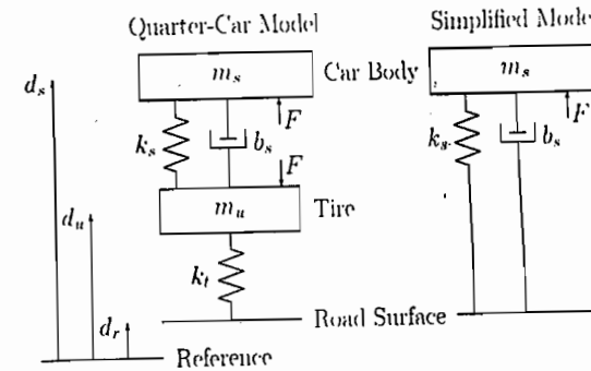
Figure 11.4: Quarter-Car Model of Automotive suspension.
