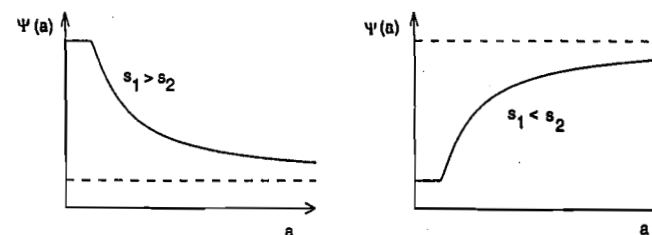
Figure 7.16: Describing function for the piecewise-linear function of Figure 7.15.
