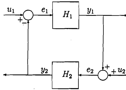
Figure 5.1: Feedback connection.
