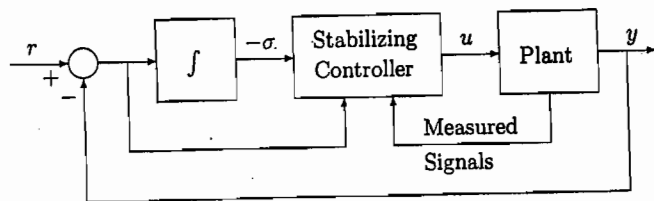
Figure 12.1: Integral control.
