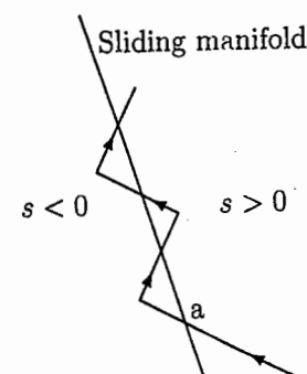
Figure 14.3: Chattering due to delay in control switching.
