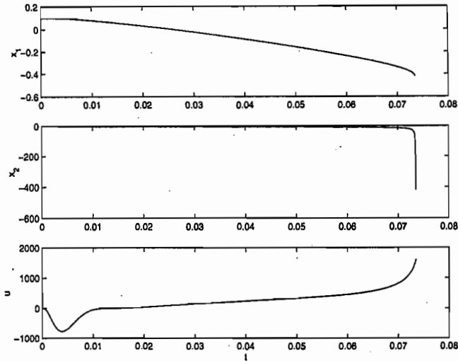
Figure 14.17: Instability induced by peaking at \varepsilon = 0.004 .
