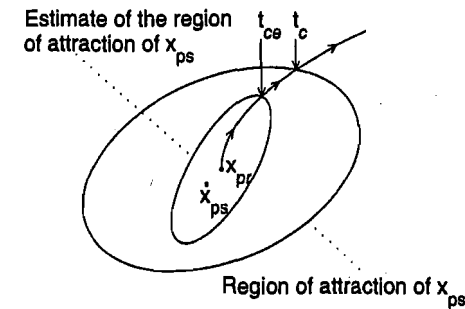
Figure 8.1: Critical clearance time.
