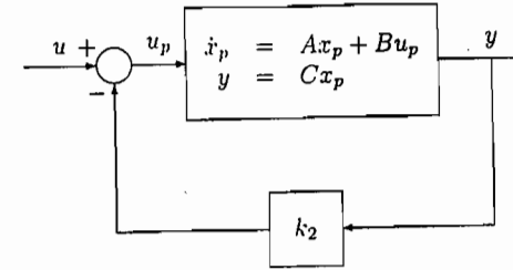
Figure 11.2: Simplified block diagram of Figure 11.1.
