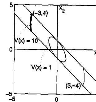
Figure 8.5: Estimates of the region of attraction for Example 8.10.
