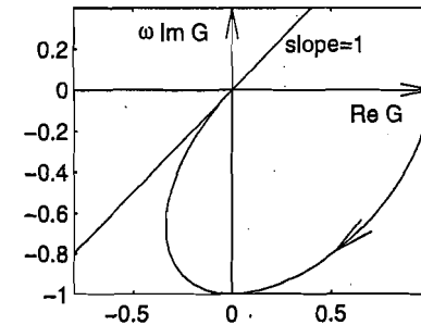
Figure 7.14: Popov plot for Example 7.5.
