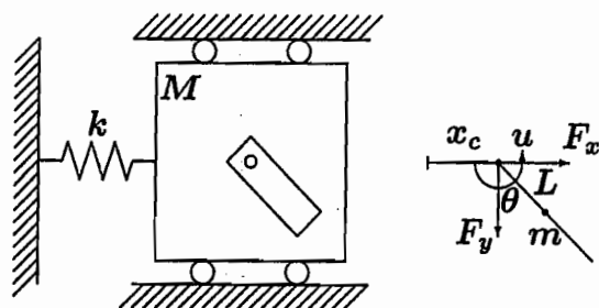
Figure 1.25: Translational Oscillator with Rotating Actuator (TORA) system.
