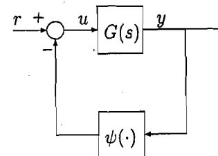
Figure 7.1: Feedback connection.
