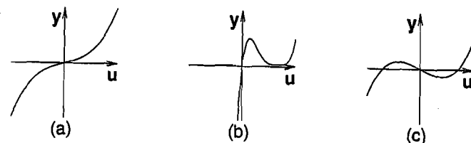
Figure 6.2: (a) and (b) are examples of nonlinear passive resistor characteristics; (c) is an example of a nonpassive resistor.
