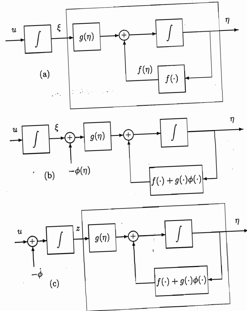
Figure 14.15: (a) The block diagram of system (14.49)–(14.50); (b) introducing \phi(\eta) ; (c) "backstepping" -\phi(\eta) through the integrator.
