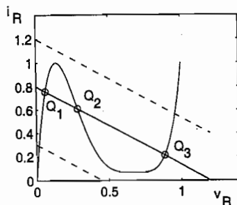
Figure 1.3: Equilibrium points of the tunnel-diode circuit.
