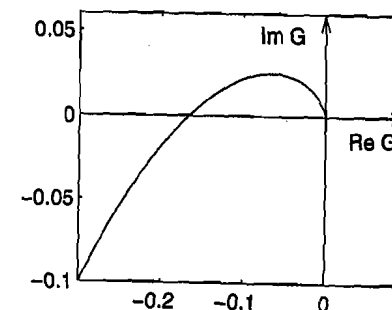
Figure 7.17: Nyquist plot for Example 7.12.
