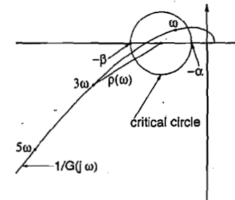
Figure 7.19: Finding \rho(\omega) .
