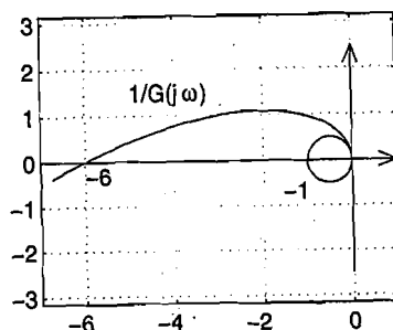
Figure 7.22: Inverse Nyquist plot and critical circle for Example 7.15.
