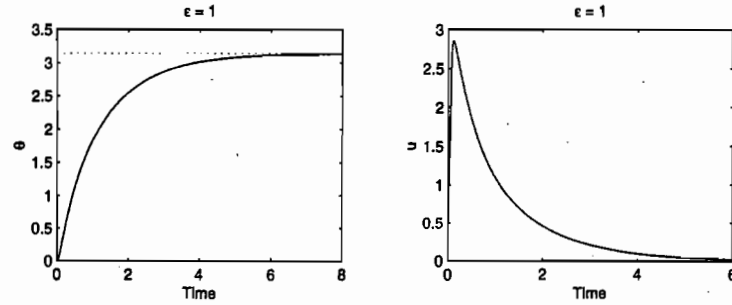
Figure 14.10: "Continuous" sliding mode control when \delta_1 = \pi .
