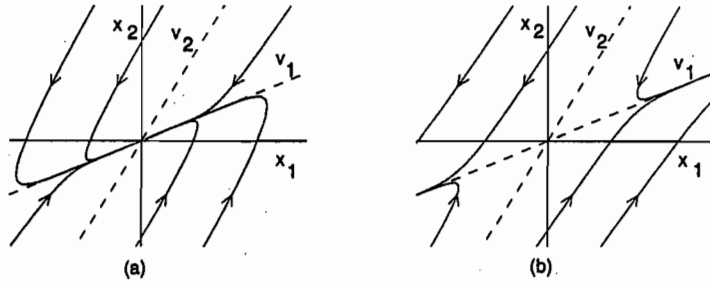
Figure 2.12: Phase portraits of a perturbed system when \lambda_1 = 0 and \lambda_2 < 0 : (a) \mu < 0 ; (b) \mu > 0 .
