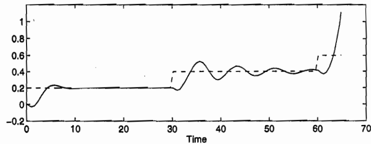
Figure 12.7: The reference (dashed) and output (solid) signals of the fixed gain controller of Example 12.6.
