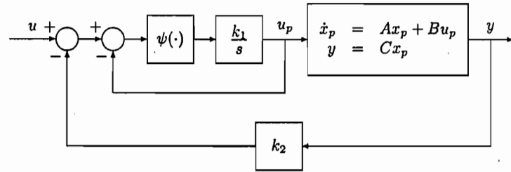
Figure 11.1: Actuator control with high-gain feedback.
