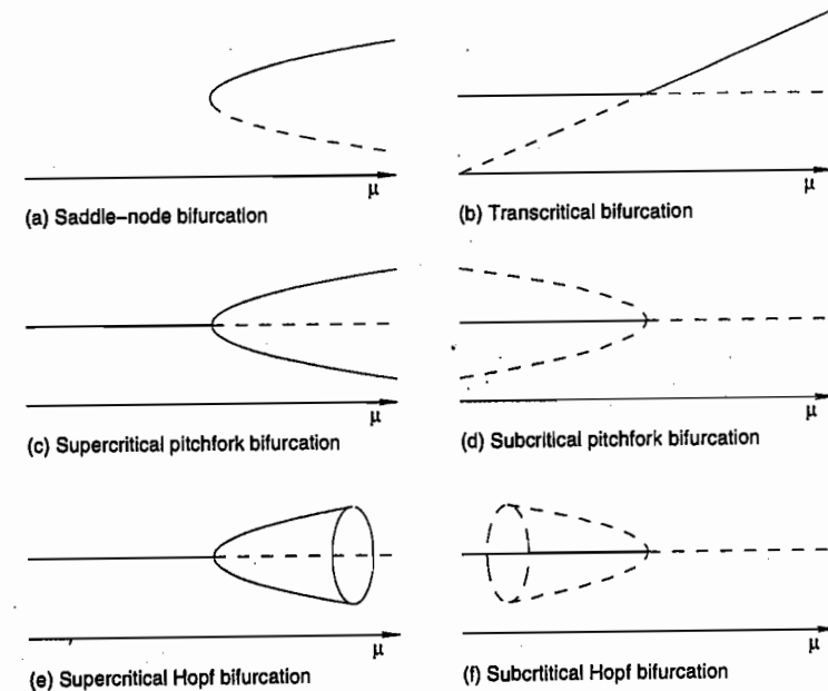
Figure 2.28: Bifurcation diagrams.
