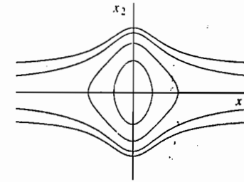
Figure 4.4: Lyapunov surfaces for V(x) = x_1^2/(1+x_1^2) + x_2^2 .
