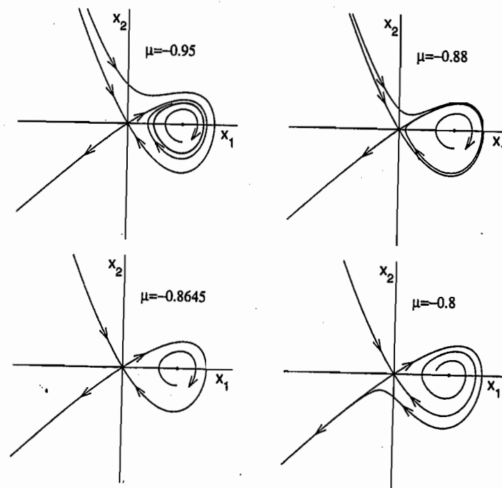
Figure 2.32: Saddle-connection bifurcation.
