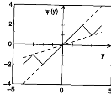
Figure 7.18: Nonlinearity of Example 7.13.
