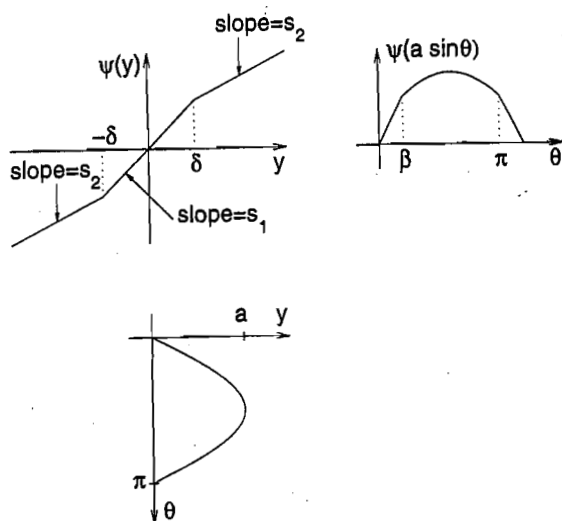
Figure 7.15: Piecewise-linear function.
