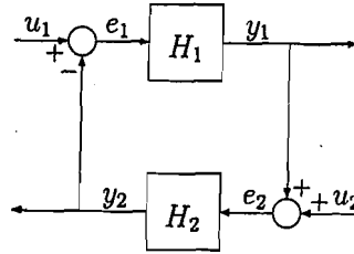
Figure 6.11: Feedback connection.
