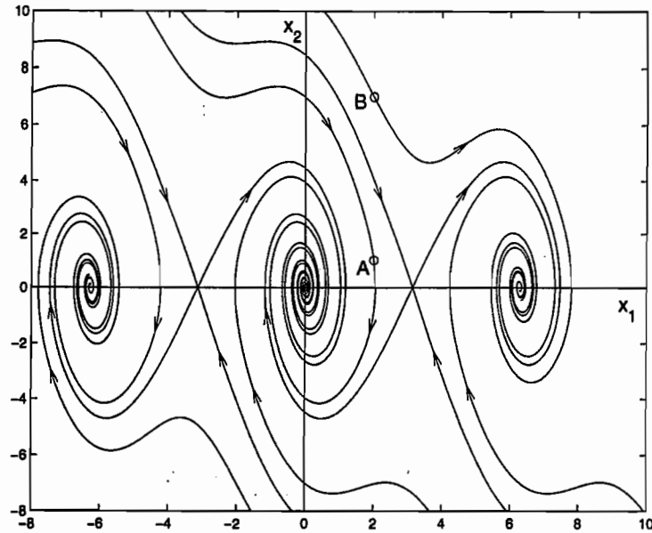
Figure 2.16: Phase portrait of the pendulum equation of Example 2.2.
