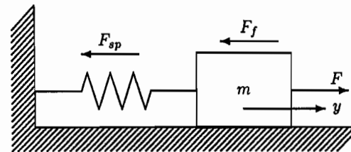
Figure 1.4: Mass-spring mechanical system.
