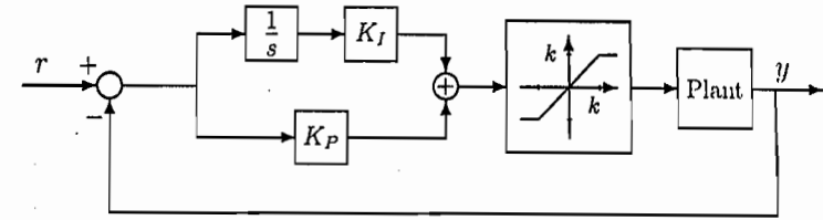
Figure 14.13: The "continuous" sliding mode controller (14.29) for relative-degree-one systems: a PI controller with K_I = kk_0/\varepsilon and K_P = k/\varepsilon , followed by saturation.
